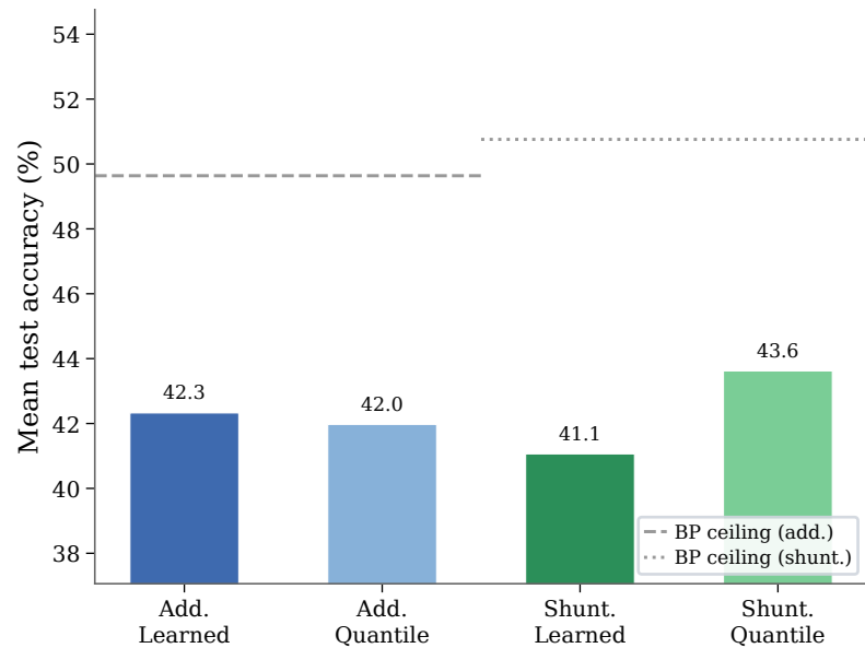
(B) CIFAR-10: LocalCA b,m update policy
