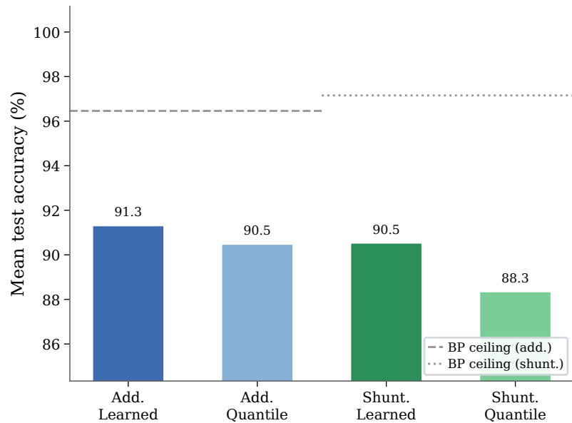
(A) MNIST: LocalCA b,m update policy
