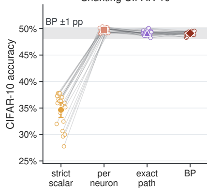
Shunting CIFAR-10
