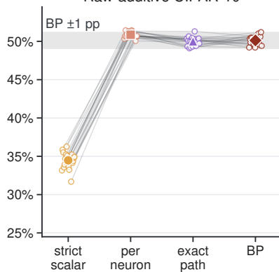
Raw-additive CIFAR-10
