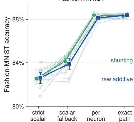
Fashion-MNIST
