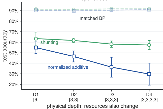
Depth stress
