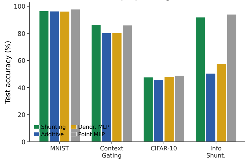
Backprop ceilings
