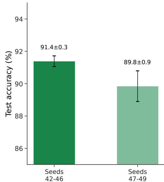
MNIST verification
