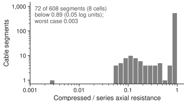
E Axial resistance after compression
