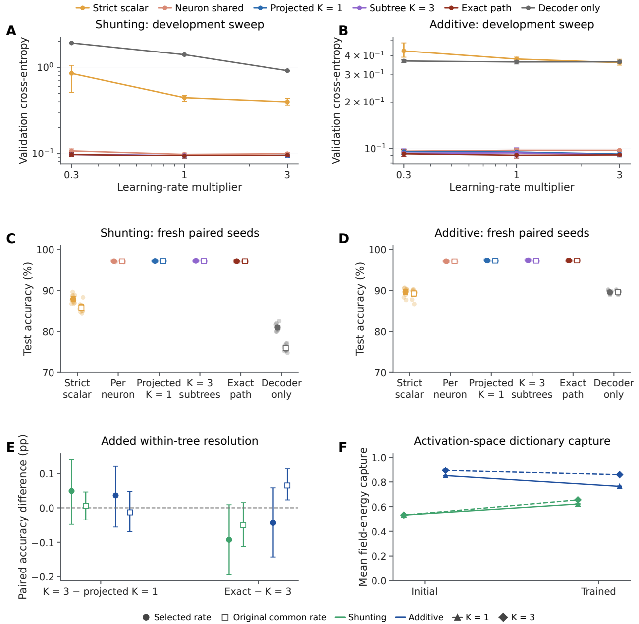
Figure S49: Intermediate subtree credit, learning-rate sensitivity and a decoder-only reference on MNIST. A,B, Development validation cross-entropy at three common multipliers of the original Adam parameter-group rates. Three development seeds per architecture, rule and multiplier give 108 fits; minimum mean validation loss selects each rule's rate. C,D, Test accuracy of ten fresh paired seeds per architecture and rule. Filled circles use selected rates; open squares use the original common rate. Small points retain all seeds; coincident rate conditions reuse one fit. The decoder-only reference trains the linear readout while preserving the initialized core. E, Paired accuracy differences from retaining three profiles instead of one, and from adding exact path resolution to the three-profile dictionary. Both projected rules acquire coefficients from the exact activation-error field, preserving the same common-mode mean at identical parameters; their field norms need not match. Green and blue identify shunting and additive networks. F, Mean field-energy capture by uniform K = 1 or subtree K = 3 profiles, before and after exact-credit training. The three-profile dictionary groups each proximal compartment with its three distal children; the one-profile control averages all 12 nonsomatic errors. Capture averages nonzero example–neuron ratios on 2,048 held-out images within each of ten seeds. Voltage-space capture is retained separately in Source Data. Symbols and bars summarize seed means and descriptive 95% bootstrap intervals. All scientific fits retain the complete MNIST protocol and 180-epoch budget, with validation-based checkpoint selection. Vertical scales differ across panels.
