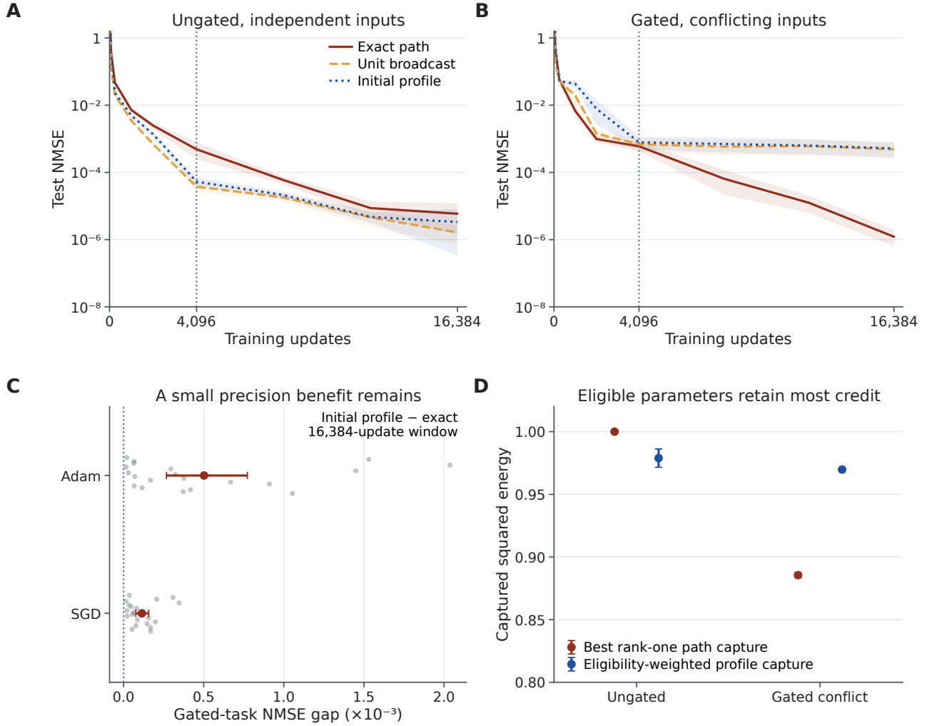
Figure S50: A first conductance task produces a small precision benefit from exact credit. A,B , Test normalized mean squared error (NMSE) at fixed checkpoints under Adam, for ungated independent inputs and gated conflicting inputs in the original 16-conductance model. Curves show means and 95% paired-seed bootstrap intervals across 20 fresh seeds; the vertical dotted line marks the original 4,096-update budget. All fits continue to 16,384 updates with unchanged optimizer and minibatch state. Unit and calibrated profiles differ here because global gradient clipping can break Adam’s invariance to fixed positive coordinate scaling. C , Gated-task NMSE differences between the initial calibrated profile and exact credit, evaluated at each fit’s best validation checkpoint in the extended window. Points are paired seed differences; symbols and bars show their means and 95% bootstrap intervals. The Adam gap is 0.000502 [0.000267, 0.000772], positive in all 20 seeds; under Adam, mean broadcast error nevertheless remains below 0.0006 NMSE. D , Diagnostics at the exact-rule best-validation states distinguish the best rank-one capture of the six-compartment path field from capture by each student’s fixed initial profile after weighting by local parameter eligibility. Both are squared-energy projection ratios with one freely fitted amplitude per example. High eligibility-weighted capture helps explain the small learning difference. The gated and ungated tasks change both inhibition and distractor dependence, so this first study is a task-family comparison. All 216 development fits, 240 fresh fits and their continuations are retained in Source Data.
