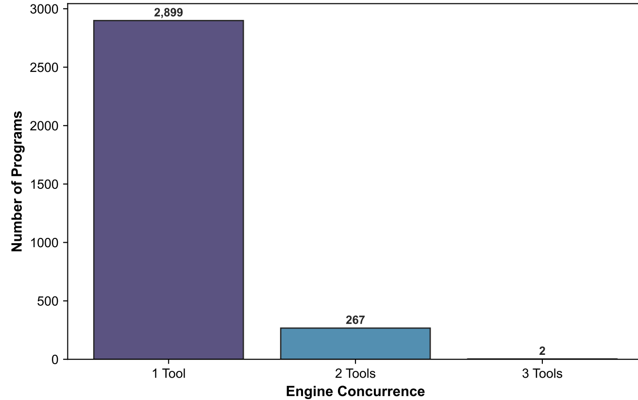
B: Static Inter-Tool Program Agreement
