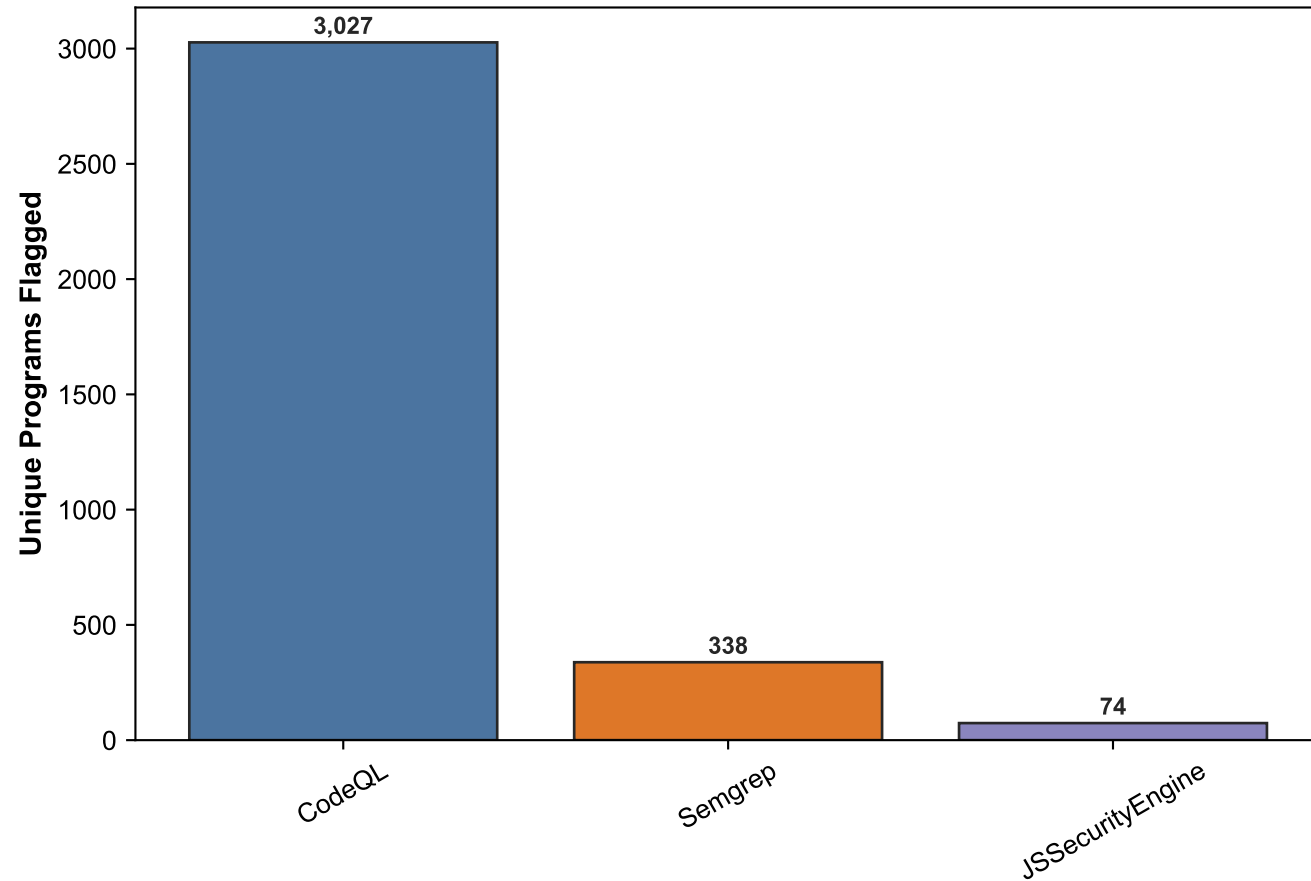
A: Programs Flagged by Static Engine
