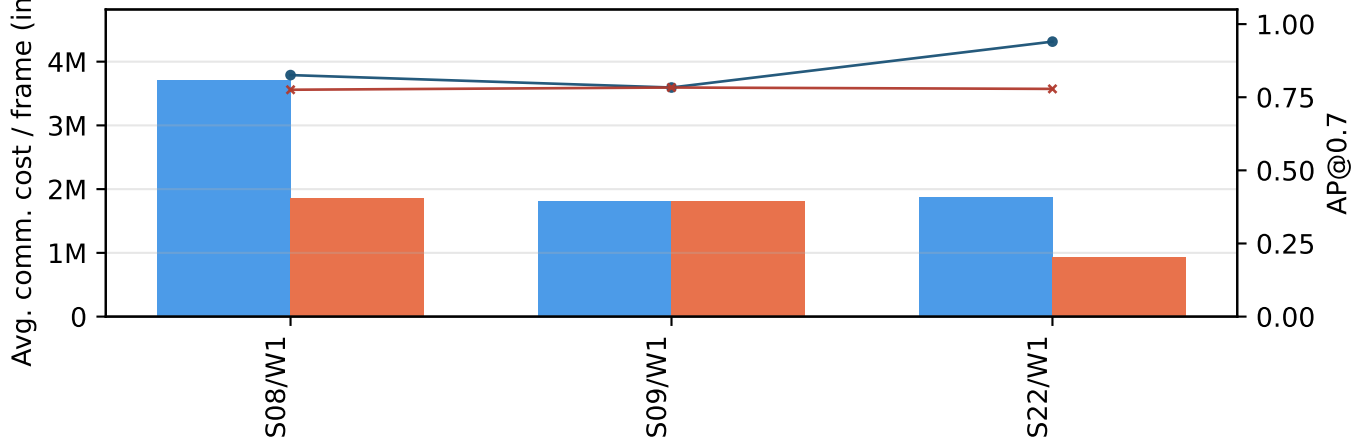
Intermediate fusion
