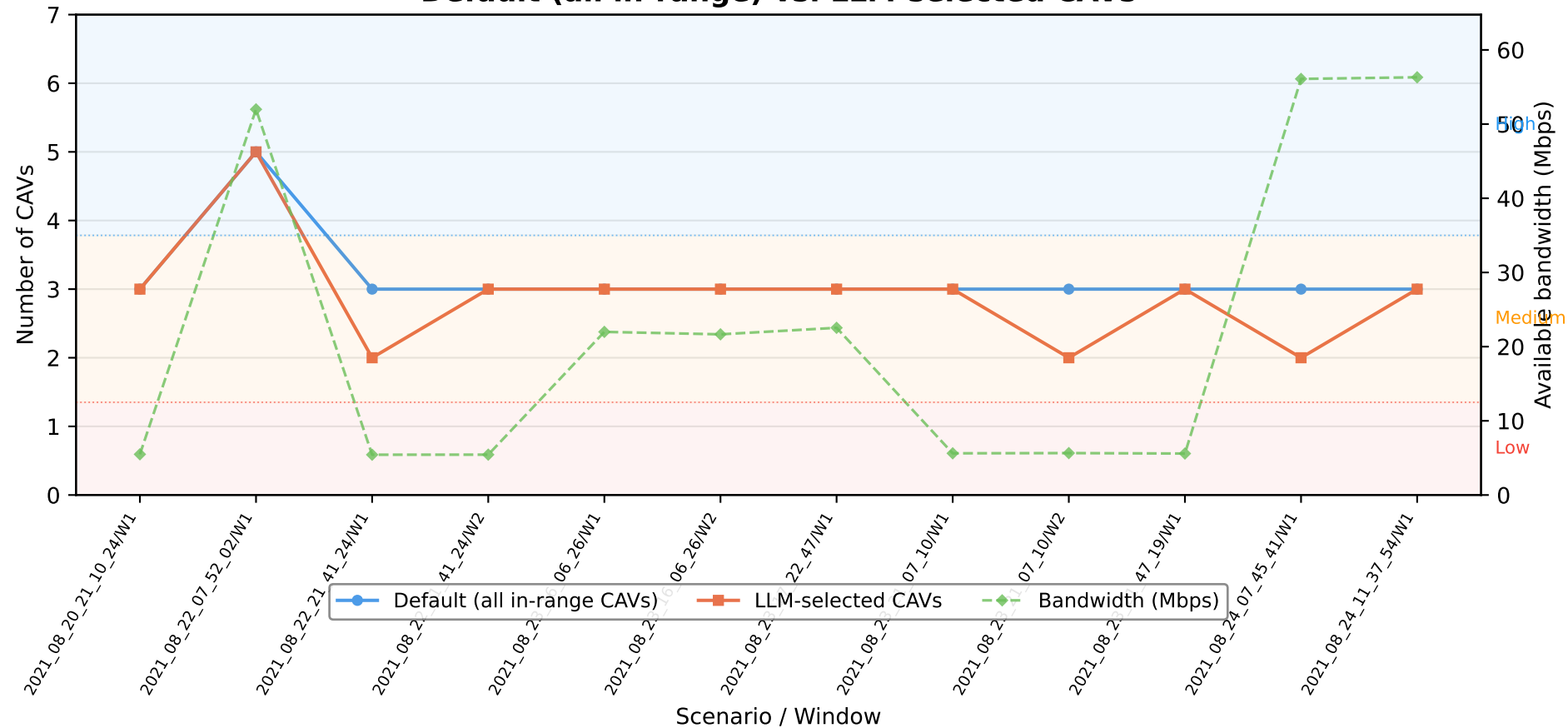
Default (all in-range) vs. LLM-selected CAVs
