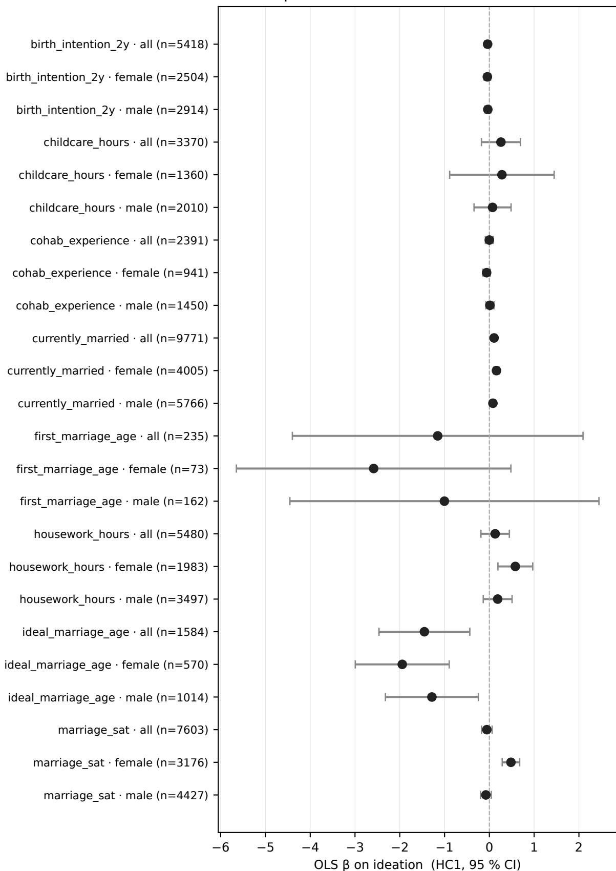
OLS \beta on ideation — CFPS 2020 cross-section
