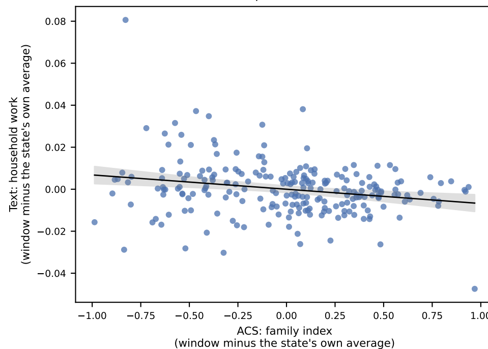
Within states — household: one point = one state-window r = -0.23 ( p = 0.001 ), n = 228
