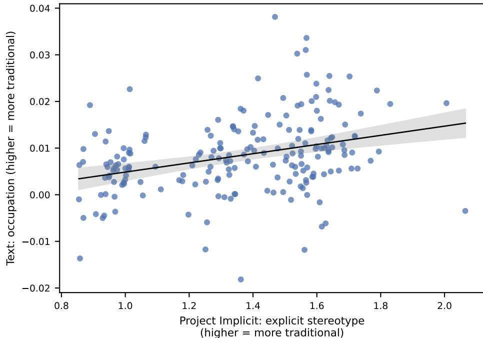
A. occupation r = 0.33 ( p = 0.000 ), n = 199
