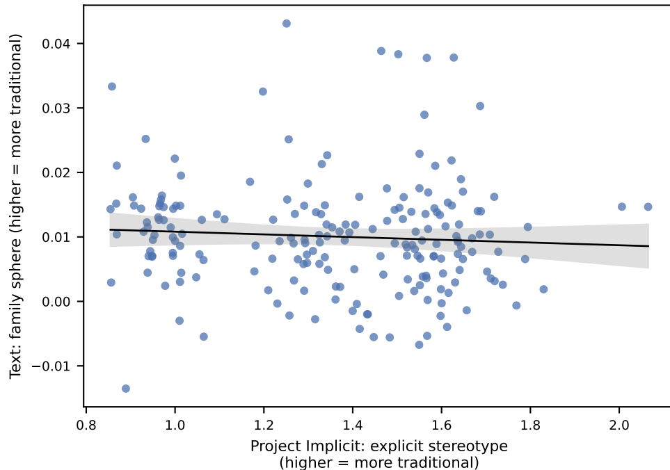
B. family r = -0.07 ( p = 0.349 ), n = 199
