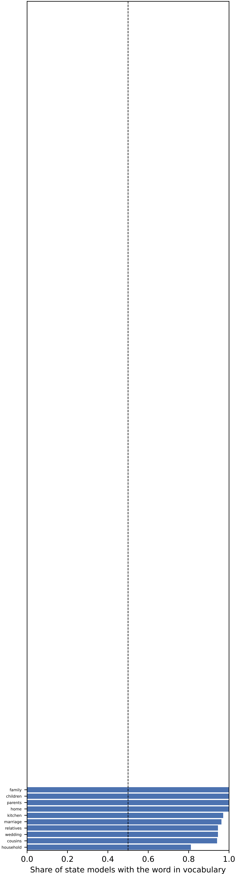
family_sphere: 10/10 used
