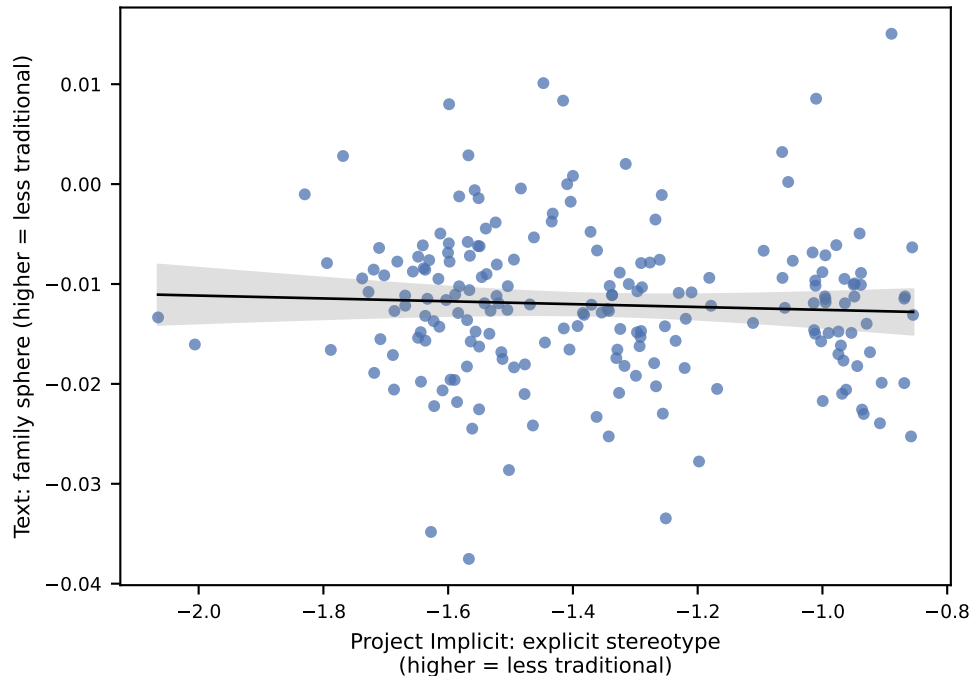
B. family: one point = one state in one 10-year window r = -0.05 ( p = 0.474 ), n = 199
