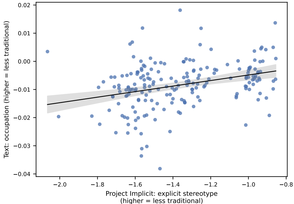
A. occupation: one point = one state in one 10-year window r = 0.33 ( p = 0.000 ), n = 199
