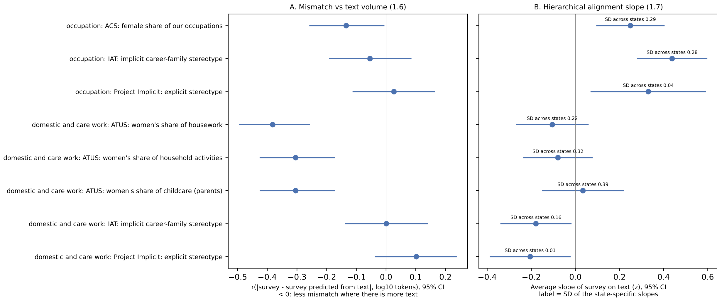
Figure 3. Measurement reliability, every direct benchmark (state-level slopes: validation-*/figures/1_7_state_slopes.pdf)
