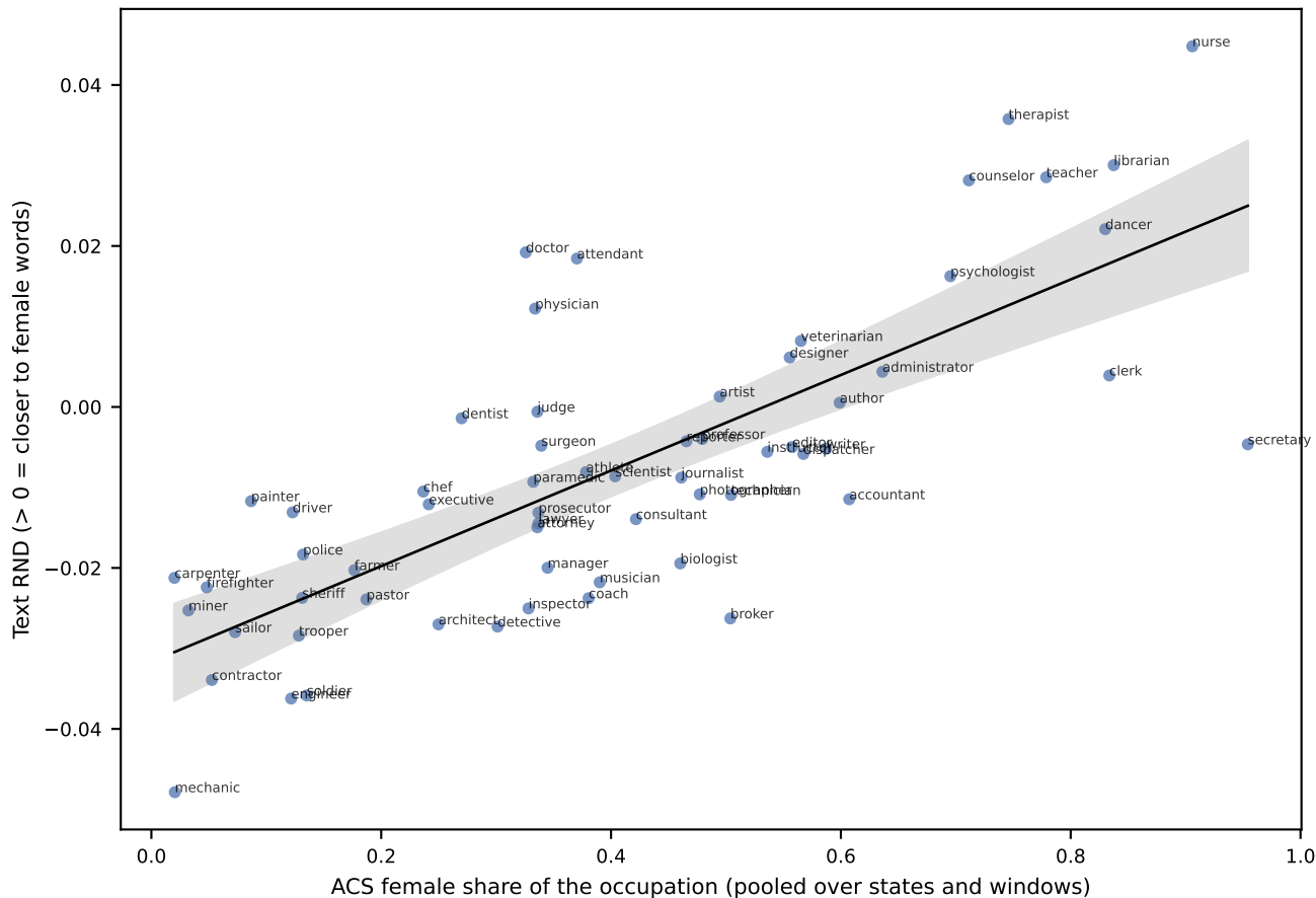
1.1 Occupations: text gender association vs female share r = 0.75 ( p = 0.000 ), Spearman \rho = 0.74 ( p = 0.000 ), n = 62
