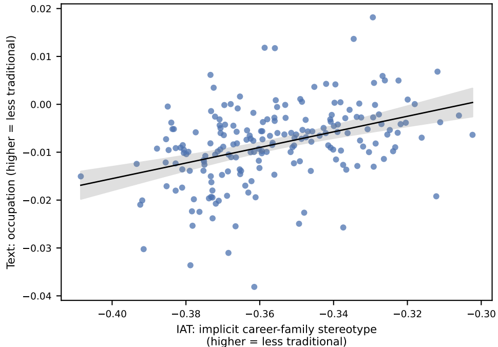
A. occupation: one point = one state in one 10-year window r = 0.41 ( p = 0.000 ), n = 199
