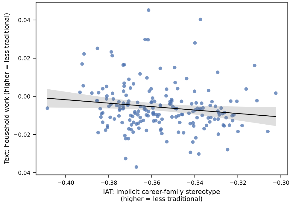
B. family: one point = one state in one 10-year window r = -0.15 ( p = 0.032 ), n = 198
