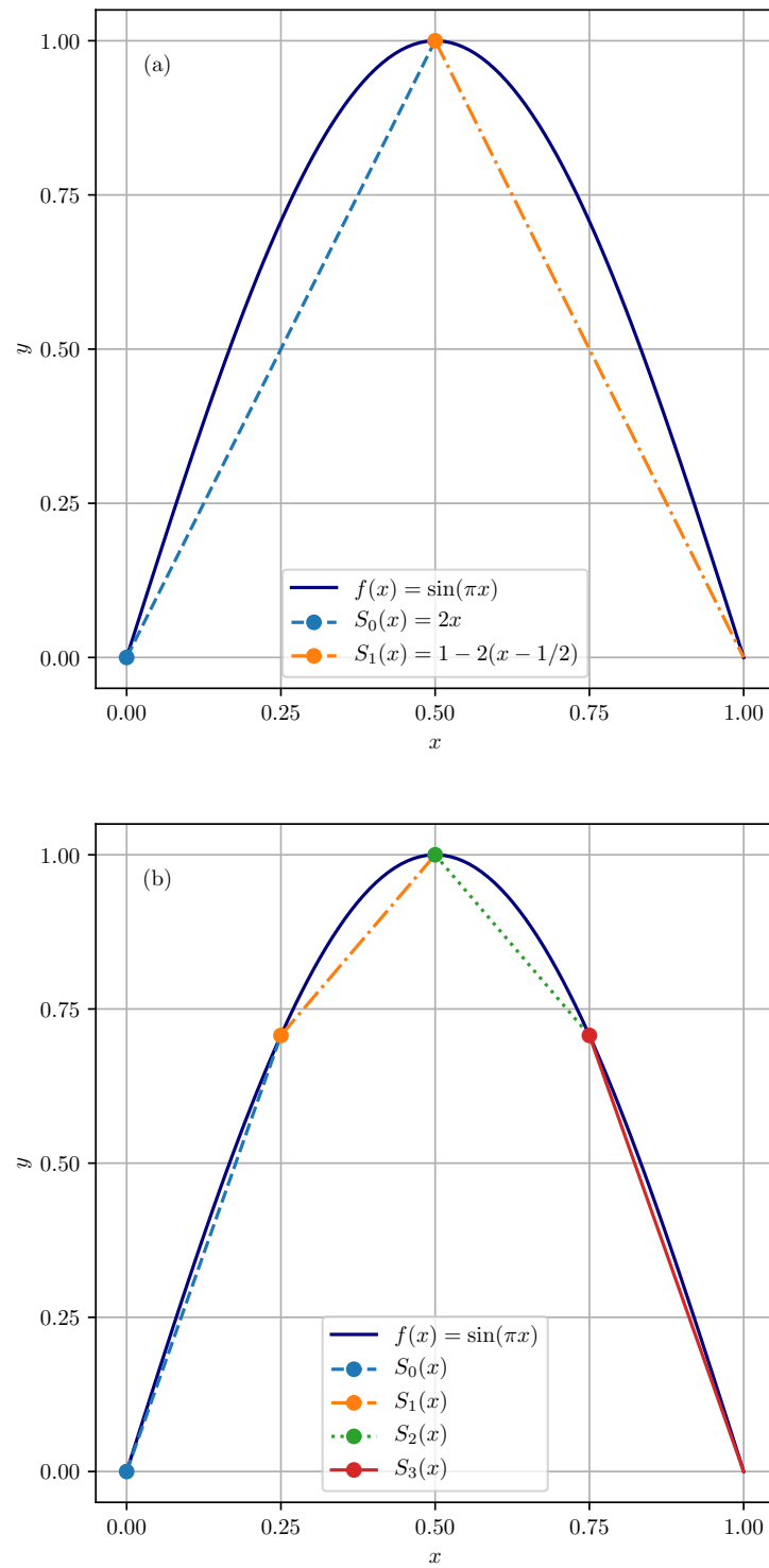
Figure 2.3: Linear spline example (a) with three points and (b) with five points, see Table 2.4 for individual definitions of S_i(x) . Reference: fig/linear_spline.py
