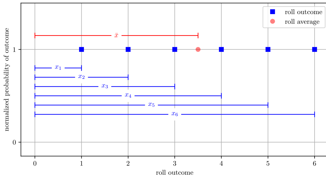
Figure 1.2: Graphical interpretation of the simple average as the first moment center of mass \bar{x} .
