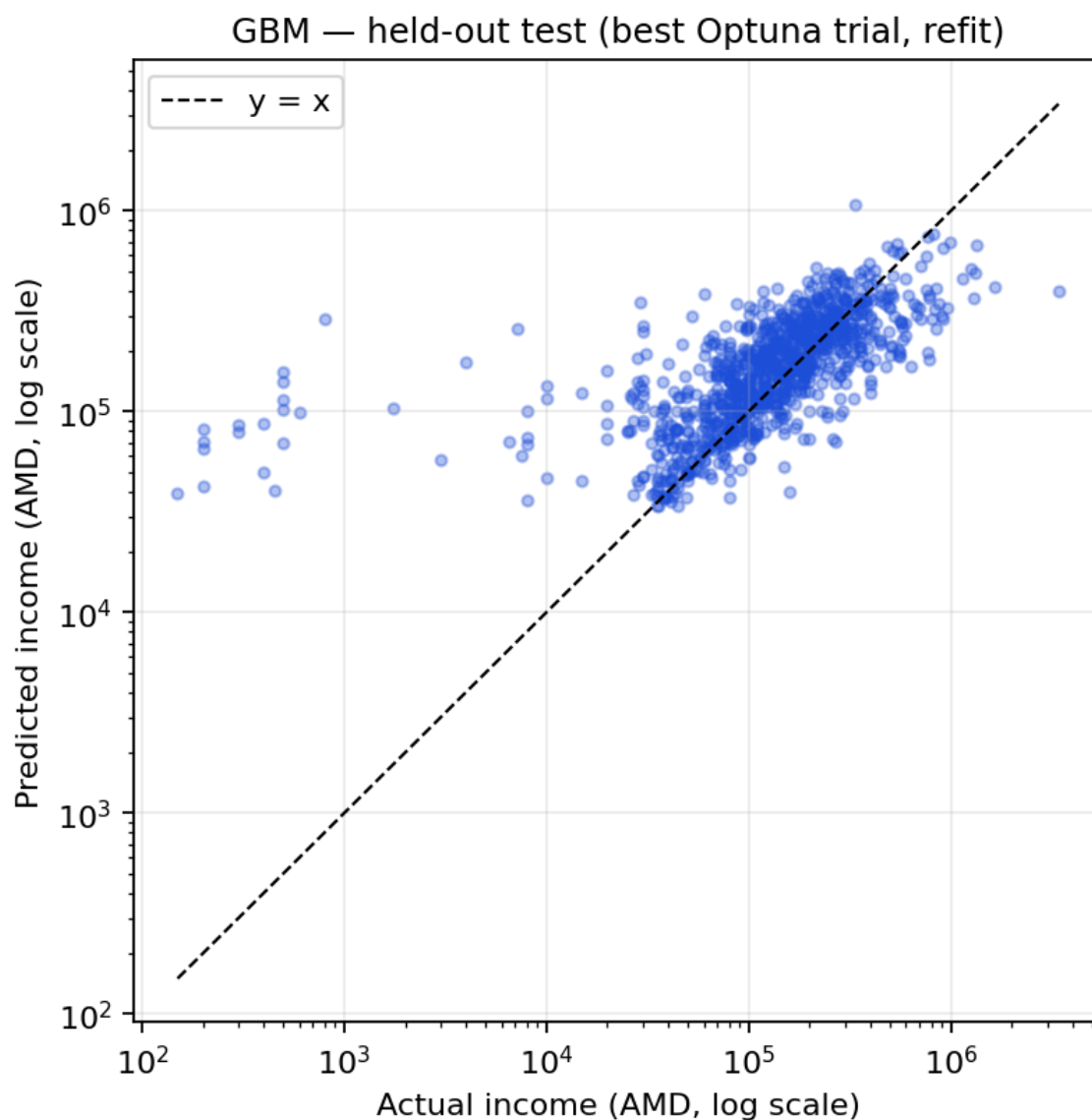
Figure 4: Predicted vs. actual household income for the tuned GBM (log–log recommended). Not on the web app —export from the same notebook as the Optuna run. See Appendix A.
