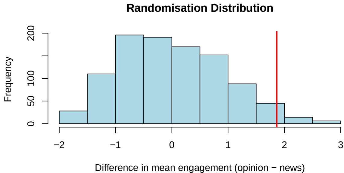
Figure 6: Randomisation distribution of the difference in means under H_0 ; the red line is the observed difference.
