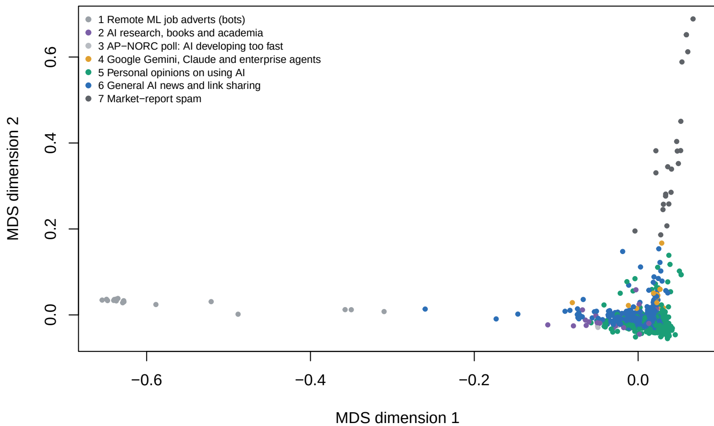
Figure 5: Posts in two MDS dimensions, coloured by cluster.
