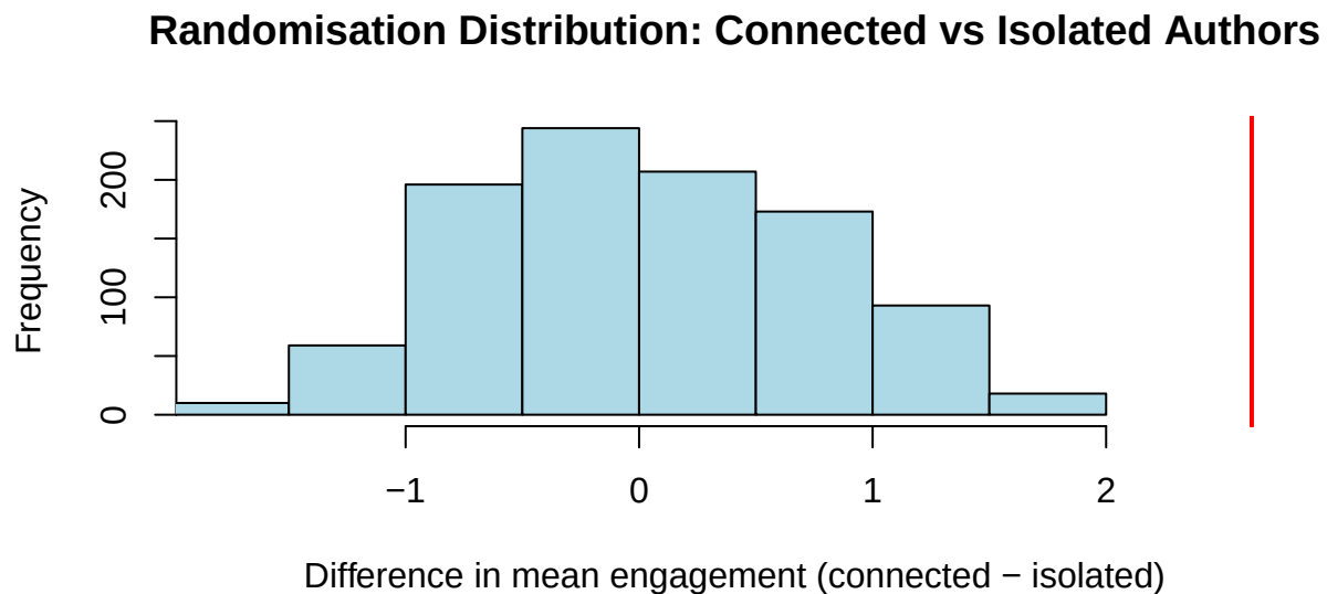
Figure 11: Randomisation distribution for connected vs isolated authors; the red line is the observed difference.
