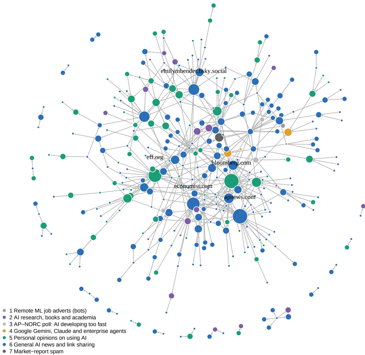
Figure 9: Full follow network of AI-post authors (authors with at least one tie).
