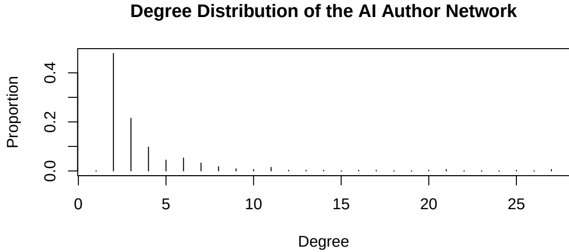
Figure 8: Degree distribution of the network.
