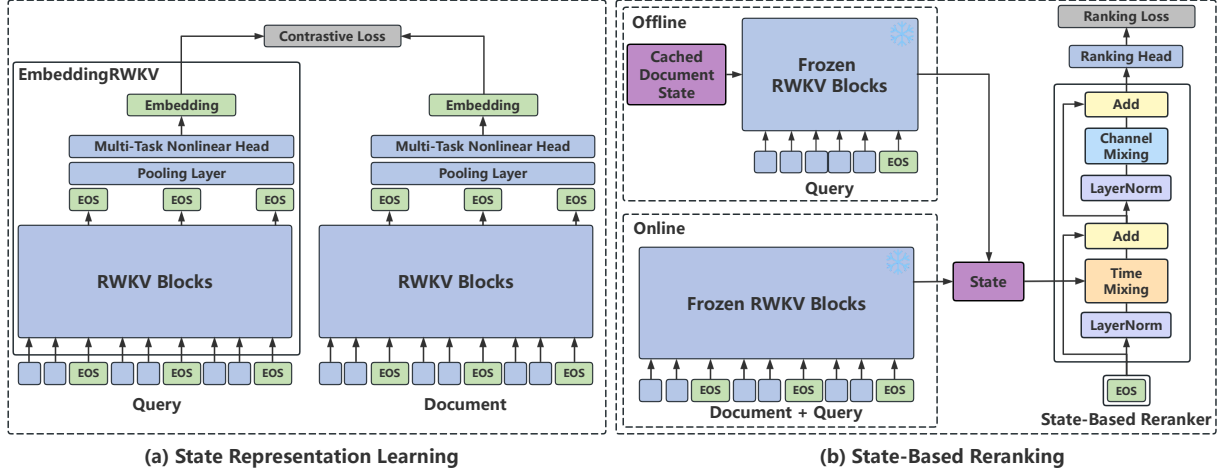
Figure 2: (a) State Representation Learning : illustrates the process of “Learning the State.” (b) State-Based Reranking : demonstrates the paradigm of “Utilizing the State” by directly reusing the cached state for inference, thereby avoiding redundant re-computation.
