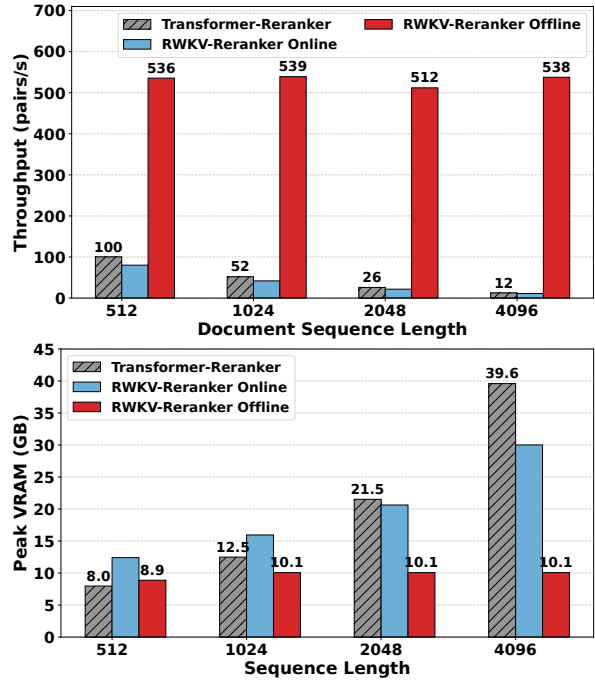
Figure 3: Performance benchmarking across various sequence lengths. Baseline: mxbai-rerank-large-v2 (1.5B) (Li et al., 2025) with FlashAttention-2 vs. Ours: EmbeddingRWKV-1.4B + RWKV-Reranker-1.3B. Top: Throughput comparison (pair/s), where higher is better. Bottom: Peak VRAM usage (GB), where lower is better.
