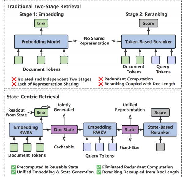
Figure 1: Traditional vs. State-Centric Retrieval. (Top) The traditional two-stage retrieval is fundamentally disjointed, suffering from redundant computation as the reranker re-encodes full document tokens. (Bottom) Our State-Centric Retrieval unifies the two stages into an efficient system via a shared, reusable state. By jointly generating embeddings and compact states, it enables offline state-based reranking that decouples inference cost from document length, yielding 5.4\times-44.8\times speedup .
