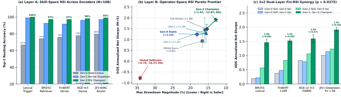
Figure 2: Empirical progression of Dual-Layer Governed Fin-RSI ( M = 5 seeds). (a) Four-generation Skill-Space RSI routing accuracy across five encoder families ( N = 108 queries, 129 skills), lifting lexical trigger Top-1 from 66.7% to 100.0% and JEV System-One to 99.1% ( \Delta m \geq 0.15 ). (b) Four-generation Operator-Space RSI Pareto trajectory on the 207,742-row balanced panel (17,886 OOS observations), contrasting monotonic governed gains against unconstrained verbal reflection. (c) Orthogonal 2 \times 2 (Skill-Space \times Operator-Space) synergy across four open-weight backbones ( p = 0.0375 ).
