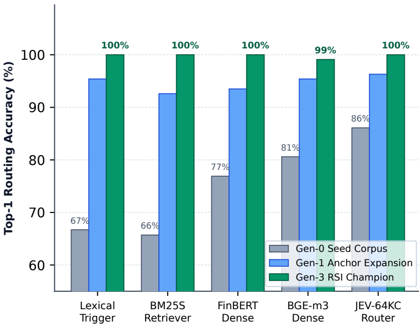
(a) Layer A: Skill-Space RSI Across Encoders (N=108)
