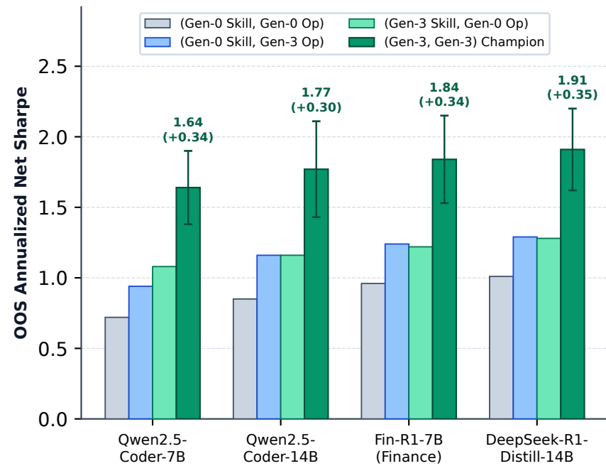
(c) 2x2 Dual-Layer Fin-RSI Synergy (p = 0.0034)
