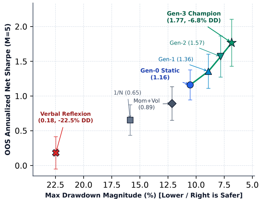
(b) Layer B: Operator-Space RSI Pareto Frontier
