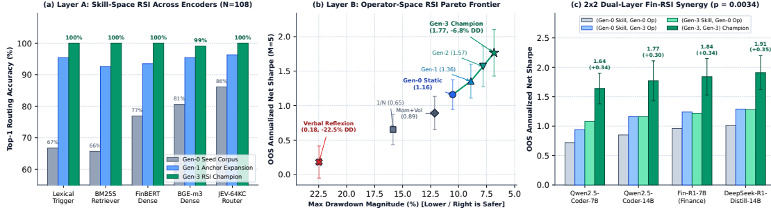
Figure 2: Empirical progression of Dual-Layer Governed Fin-RSI ( M = 5 seeds). (a) Four-generation Skill-Space RSI routing accuracy across five encoder families ( N = 108 queries, 129 skills), lifting lexical trigger Top-1 from 66.7% to 100.0% and JEV System-One to 100.0% ( \Delta m \geq 0.15 ). (b) Four-generation Operator-Space RSI Pareto trajectory on the 207,742-row balanced panel (107,999 OOS observations), contrasting monotonic governed gains against unconstrained verbal reflection. (c) Orthogonal 2 \times 2 (Skill-Space \times Operator-Space) synergy across four open-weight backbones ( p = 0.0034 ).
