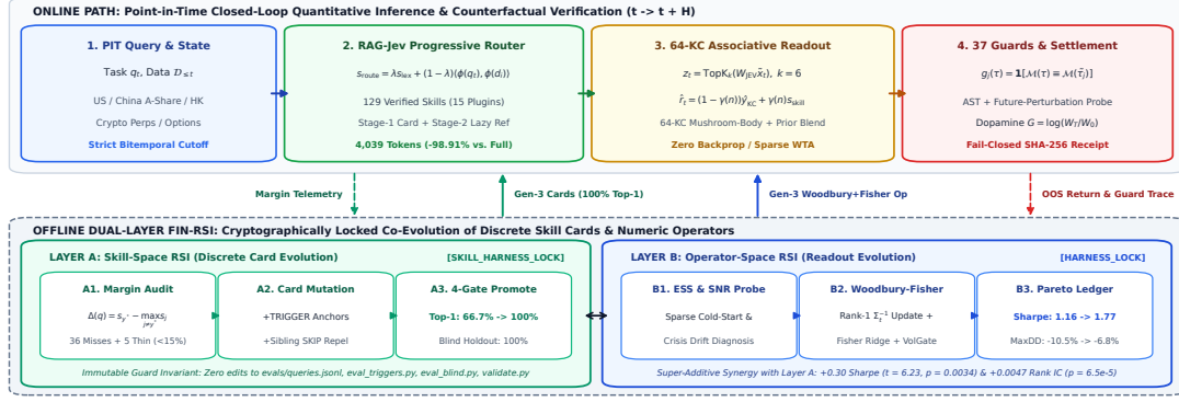
Figure 1: Architecture of the closed-loop FIN-SKILLS and Dual-Layer Governed Fin-RSI framework. Top (Online Inference & Verified Memory): Point-in-time progressive routing (RAG-Jev, -98.91\% tokens), 64-KC mushroom-body readout, and 37 counterfactual verification guards gating settlement-cleared return updates G = \log(W_T/W_0) . Bottom (Offline Dual-Layer Governed Evolution): Under SHA-256 locks, Skill-Space RSI (SKILL_HARNESS_LOCK) evolves contrastive TRIGGER/SKIP margins ( \Delta m \geq 0.15 , |d_k| \leq 1,024 ) and one-hop cross-references, while Operator-Space RSI (HARNESS_LOCK) optimizes bounded value-space pooling, James–Stein shrinkage, and rank-1 Woodbury–Fisher covariance updates under a three-way Pareto gate.
