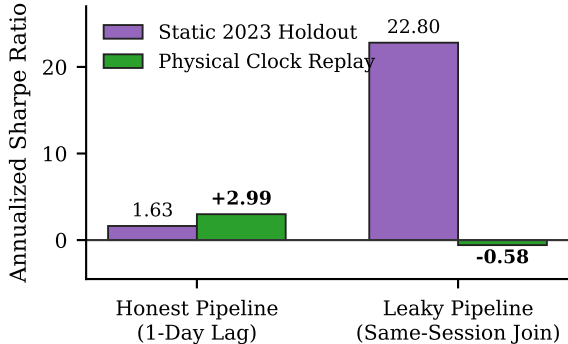
(b) Static Holdout vs. Live Clock Replay
