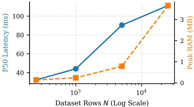
(a) \mathcal{O}(N^{0.2637}) Sub-Linear Guard Scaling
