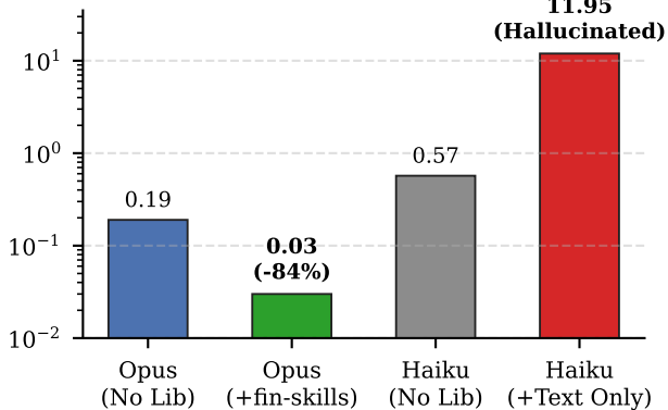
(a) Type I: Agent Compliance Paradox
