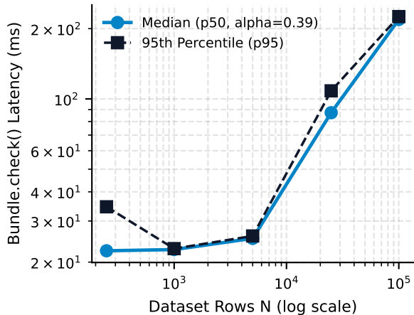
(a) Sub-Linear Guard Scaling (to N=100k)
