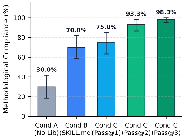
(a) FinGuardBench-60 & Self-Repair
