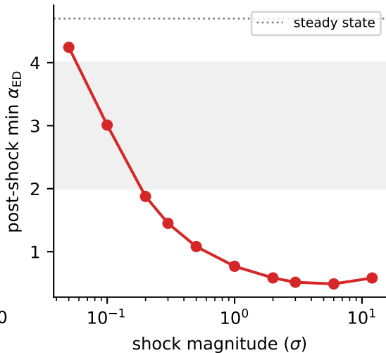
Sigmoid dose-response (5 assets)
