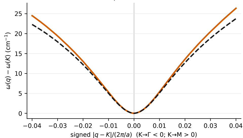
(d) K-referenced shape, 450 K near-K shape RMSE = 0.59 \text{ cm}^{-1}
