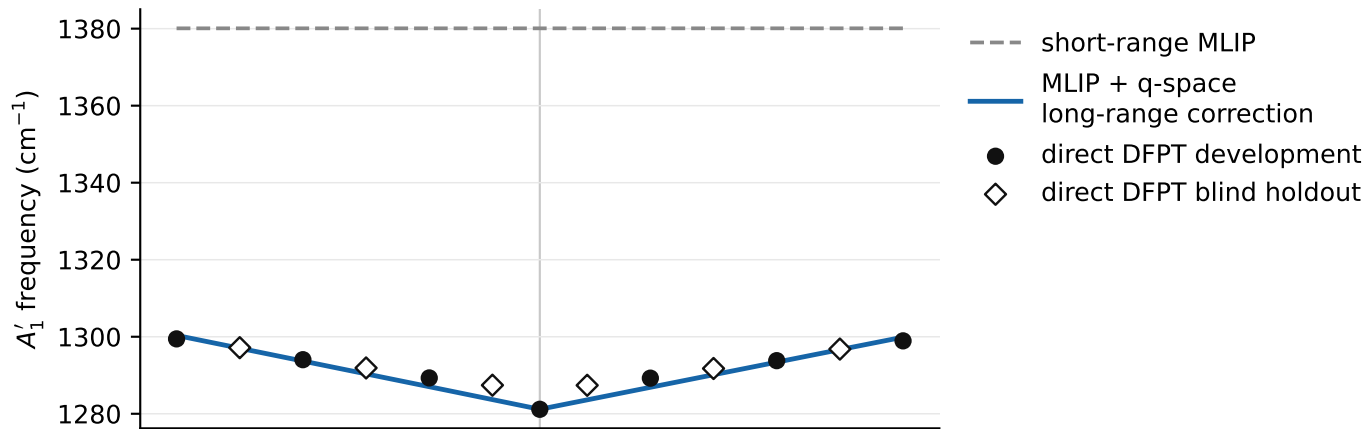
Graphene K cusp: direct DFPT vs repository method
