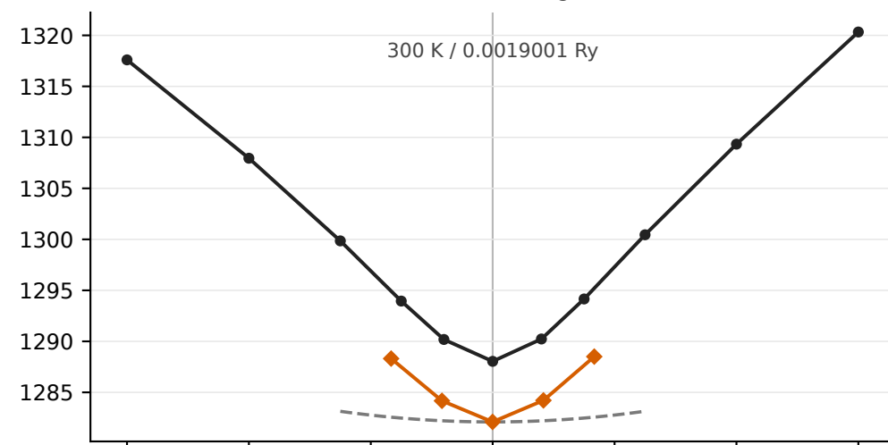
Graphene K cusp: direct DFPT and finite-lattice MLIP + q-space correction Classical TDEP background (L0) Quantum SSCHA background (Q0)
