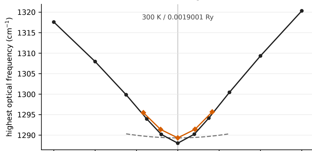
Graphene K cusp: direct DFPT and finite-lattice MLIP + q-space correction Classical TDEP background (L0) Quantum SSCHA background (Q0)
