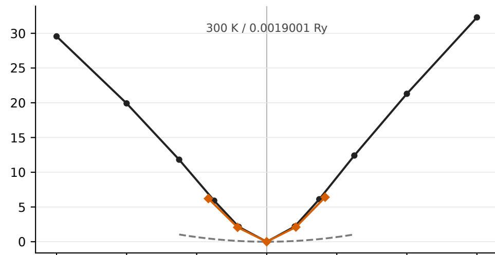
Graphene K cusp shape after removing the K-point frequency offset Classical TDEP background (L0) Quantum SSCHA background (Q0)
