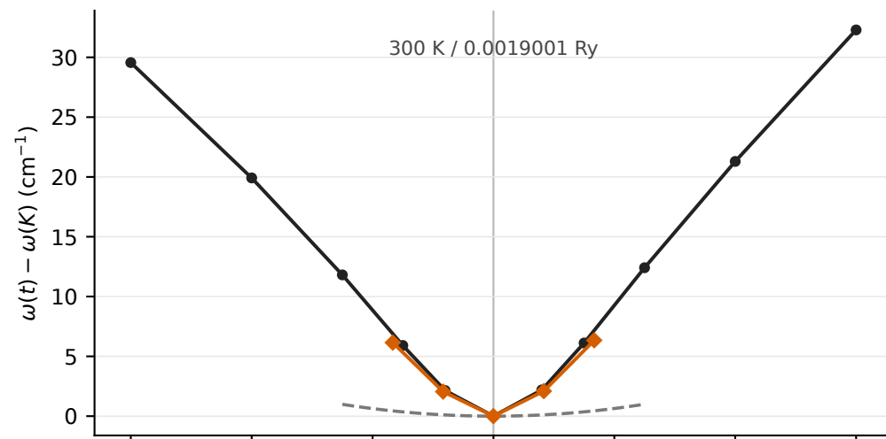
Graphene K cusp shape after removing the K-point frequency offset Classical TDEP background (L0) Quantum SSCHA background (Q0)
