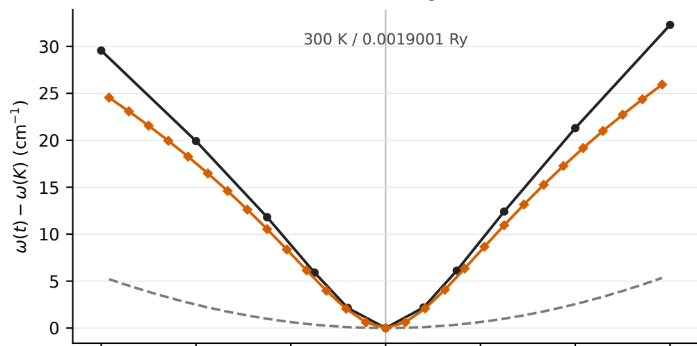
Classical TDEP background (L0)
