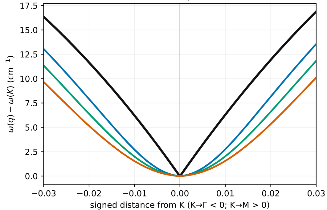
K-referenced cusp: full window
