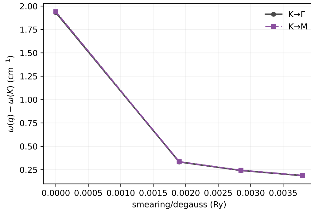
Cusp rise at |q - K| = 0.003
