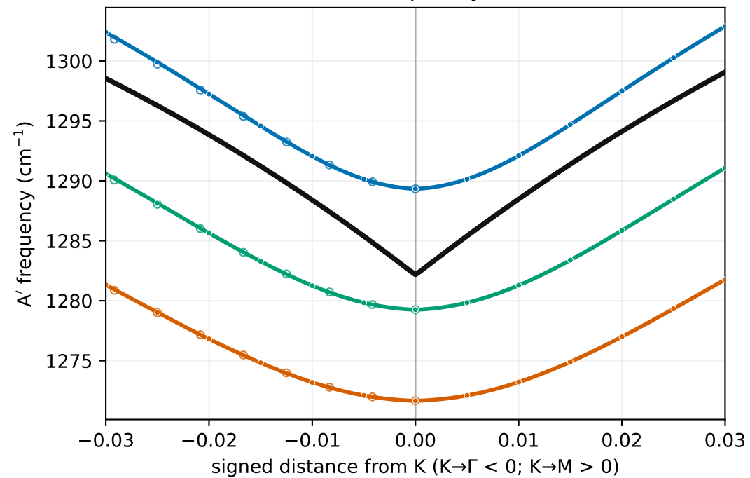
Absolute frequency: \Gamma -K-M
