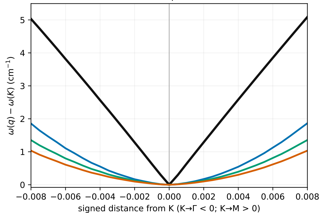
K-referenced cusp: inner window
