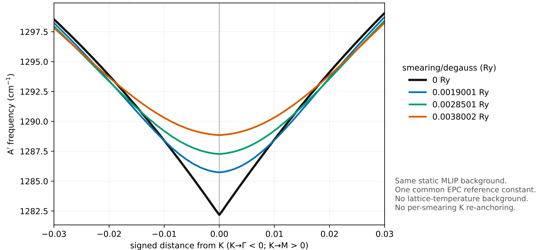
Graphene K-neighbourhood A': fixed-background absolute frequency
