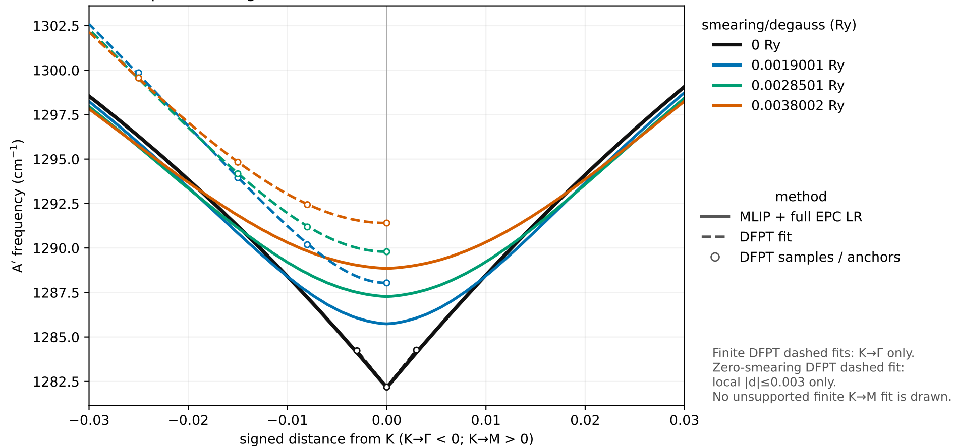
Graphene K-neighbourhood A': MLIP + full EPC LR and fitted DFPT
