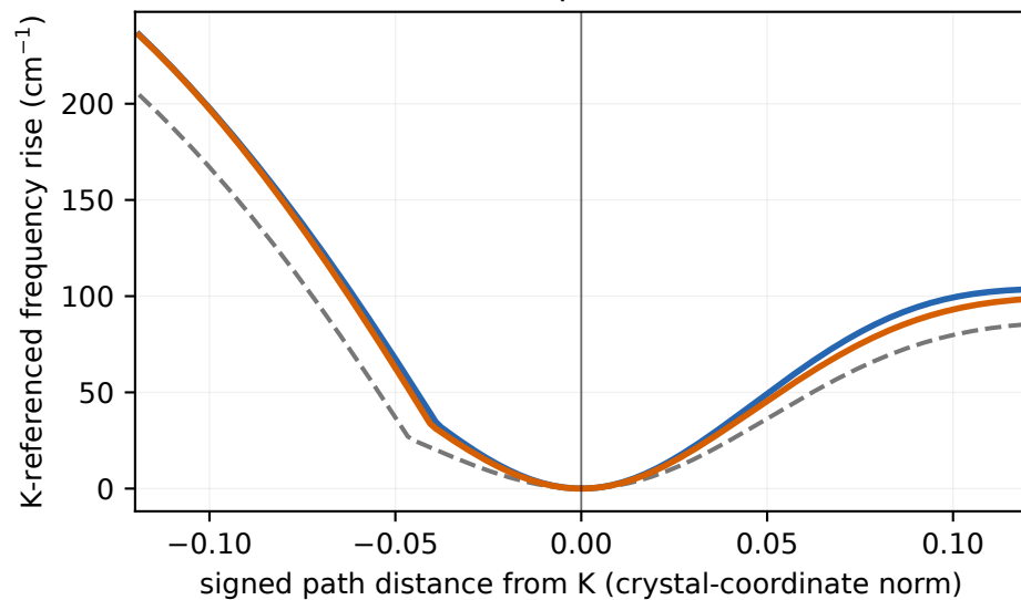
Local shape around K
