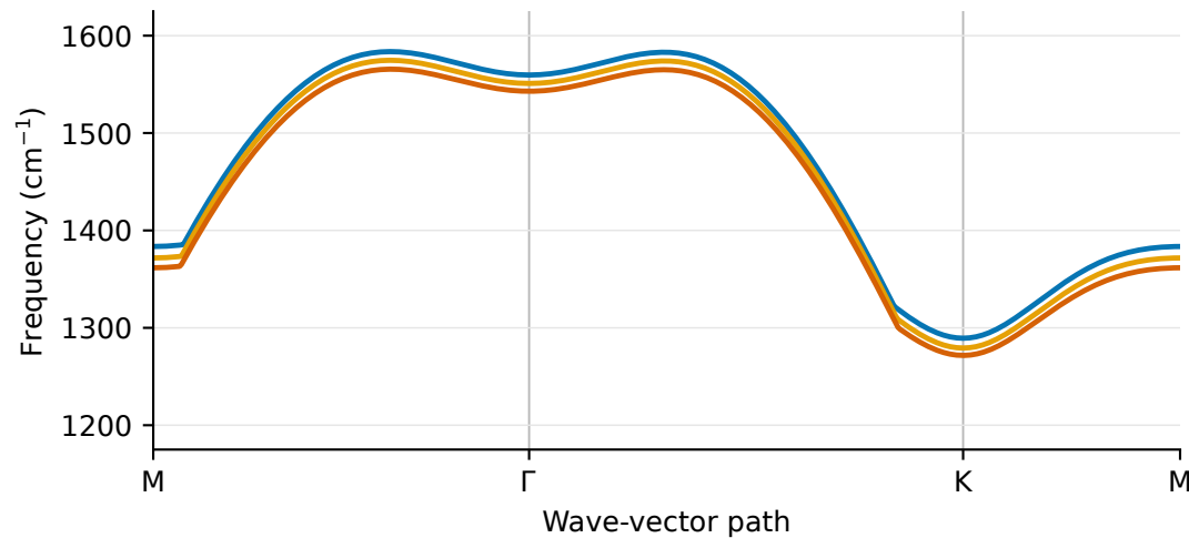
Highest optical branch
