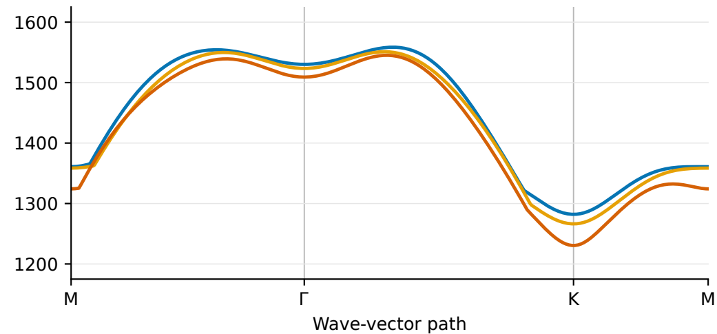
Highest optical branch
