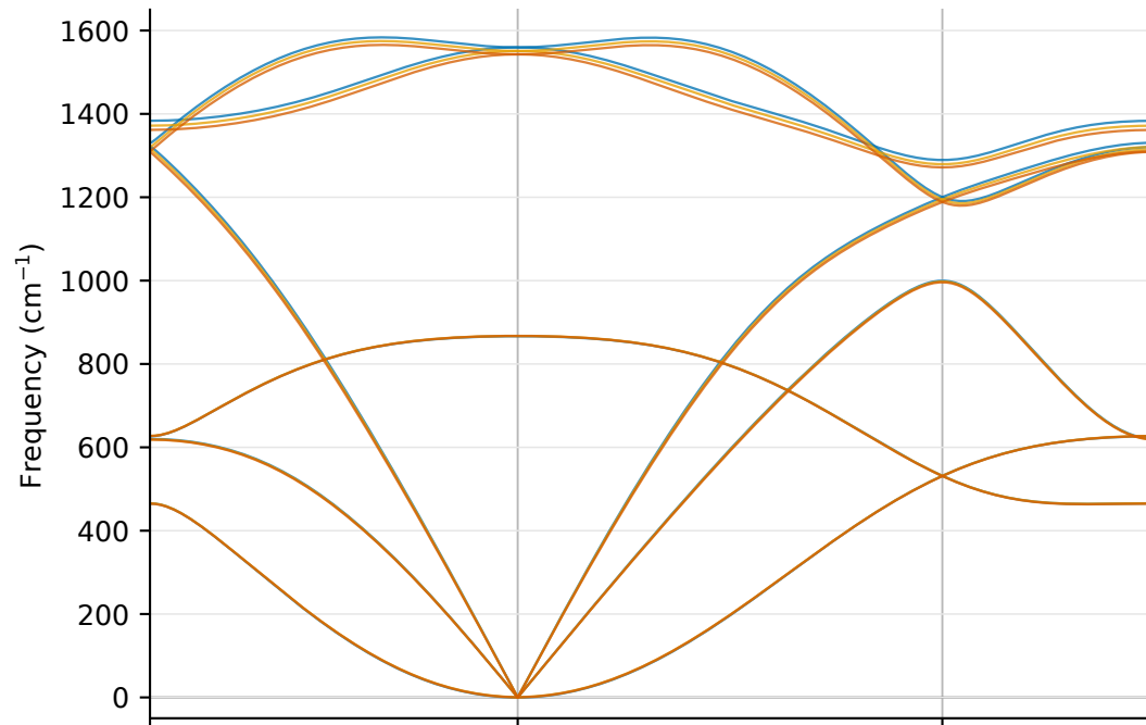
(a) Classical MD/TDEP (L0)
