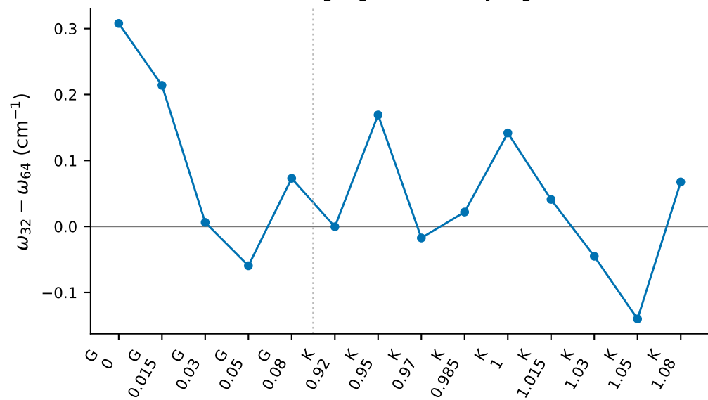
Low-smearing k-grid sensitivity ( dg=0.01 )
