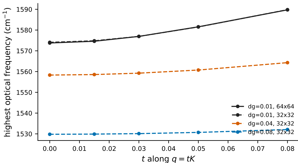
Direct DFPT Kohn-anomaly strength
