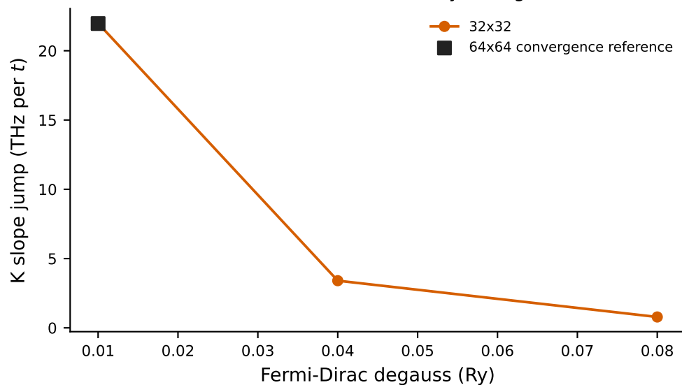
Direct DFPT Kohn-anomaly strength
