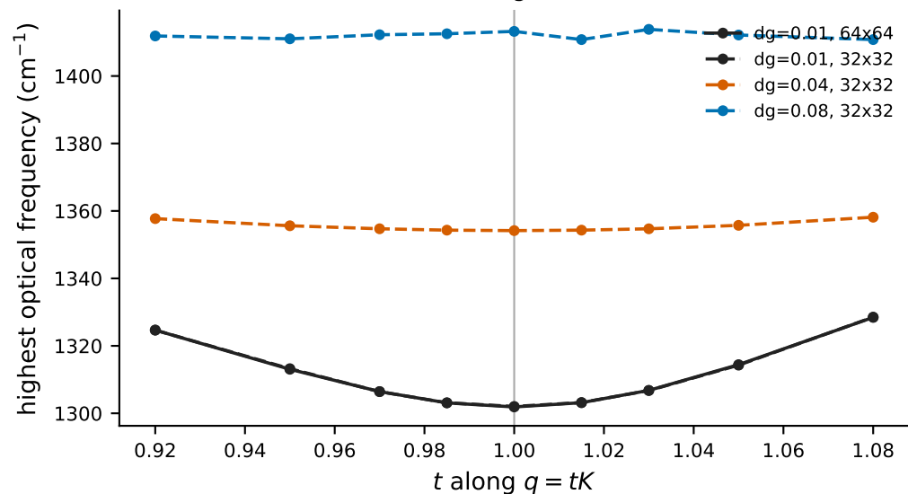
Low-smearing k-grid sensitivity ( dg=0.01 )
