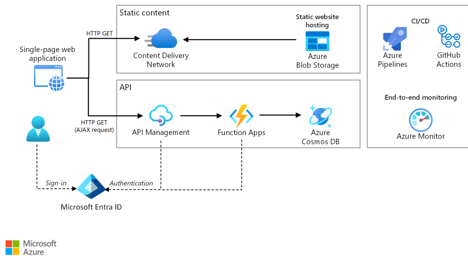
Figure 5. MS Azure Serverless Architecture[15]
