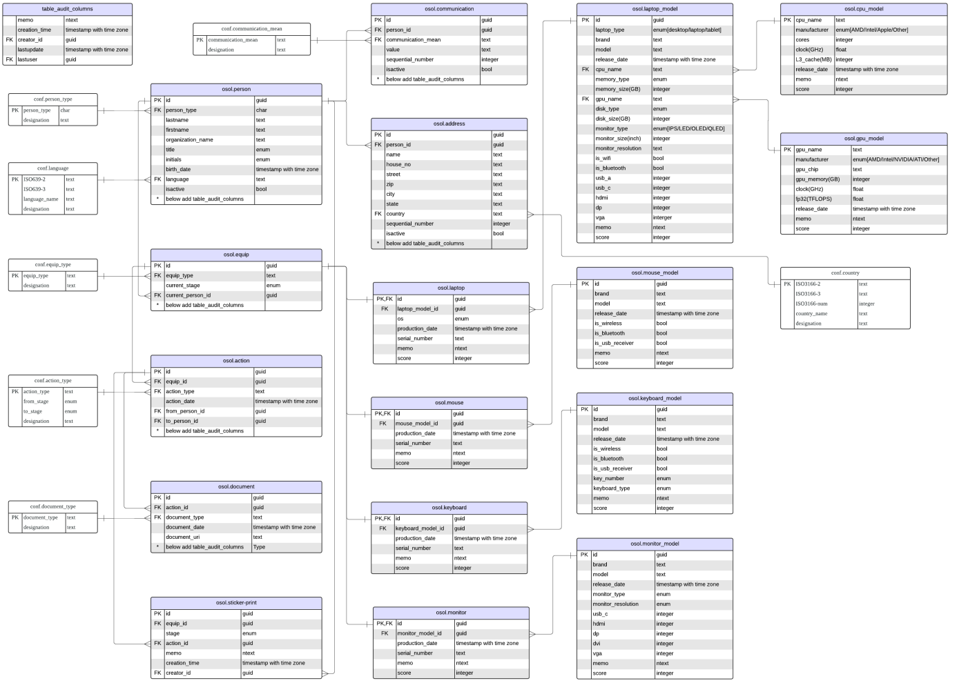
Figure 4. OSOL database schema
