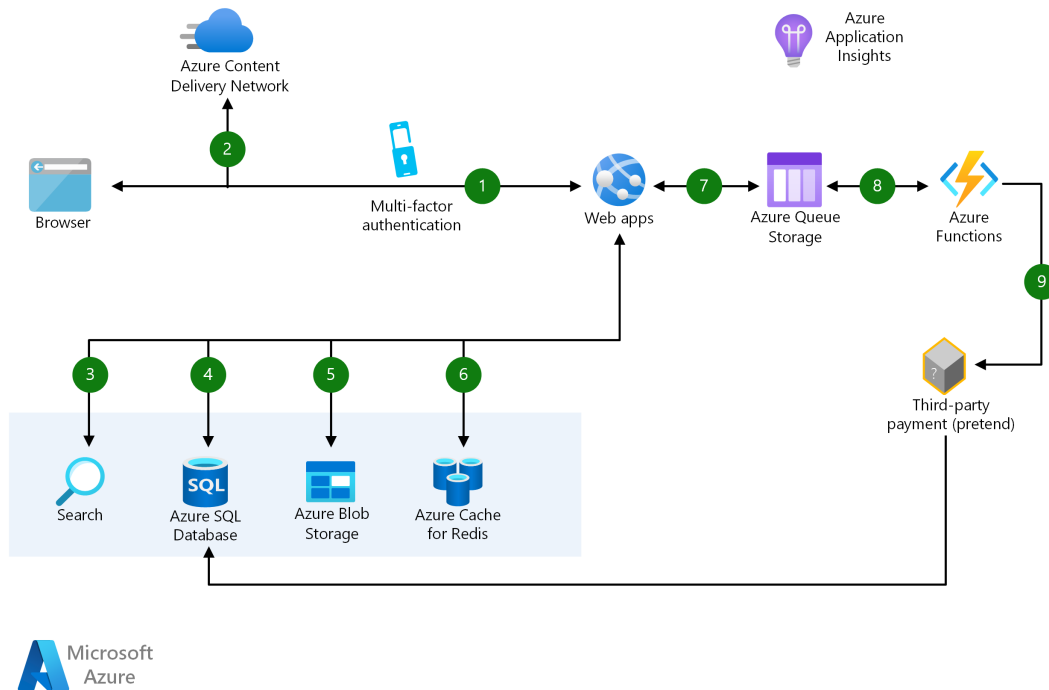
Figure 3. OSOL Tracer system draft architecture[14]
