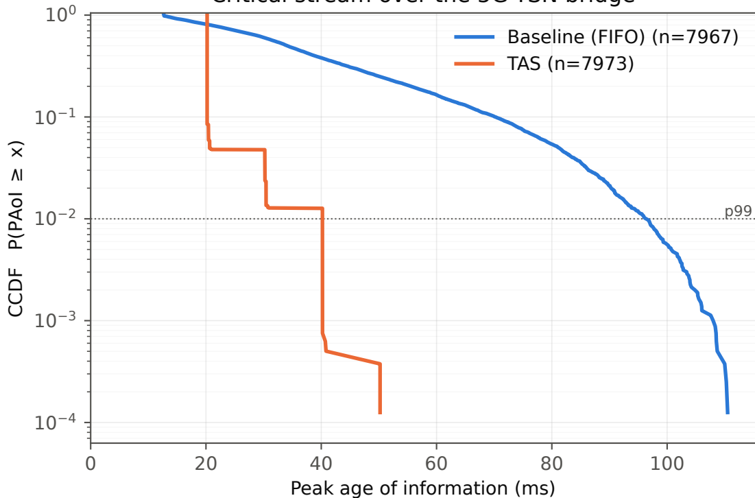
Critical stream over the 5G-TSN bridge
