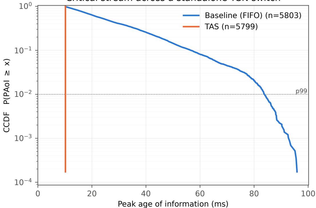
Critical stream across a standalone TSN switch
