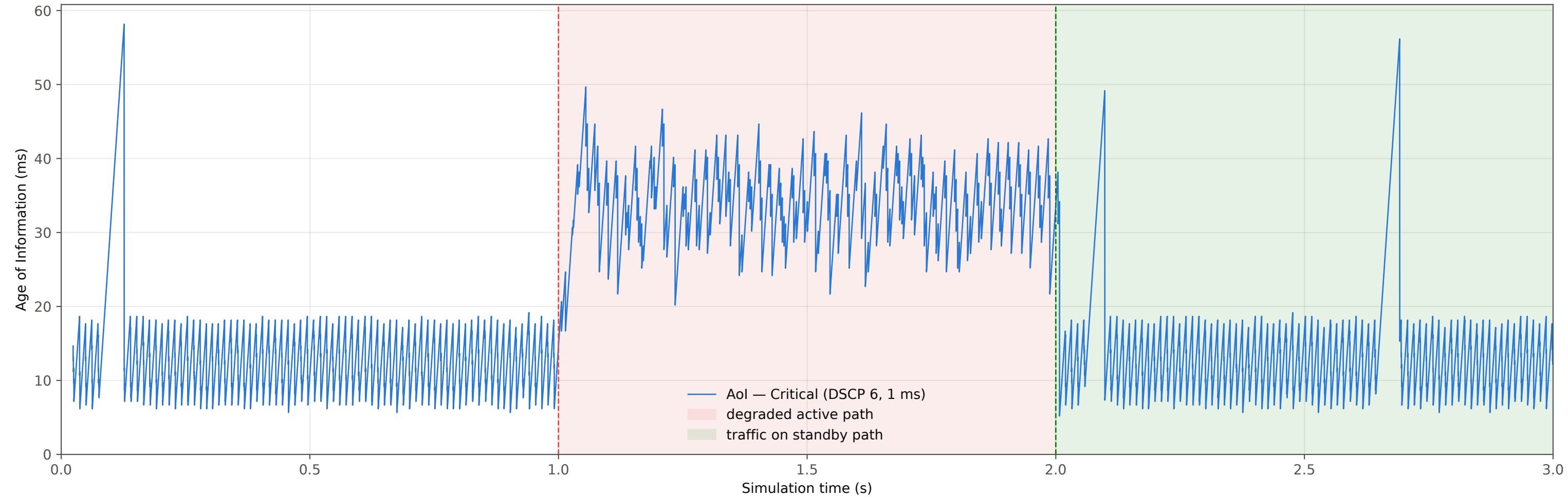
Uplink SINR degradation and failover — Critical (DSCP 6, 1 ms)
