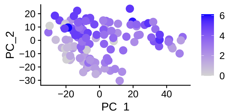
THSD7B
