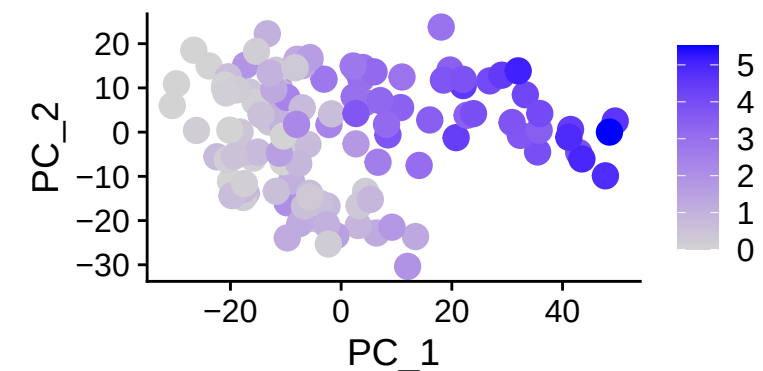
CD93
