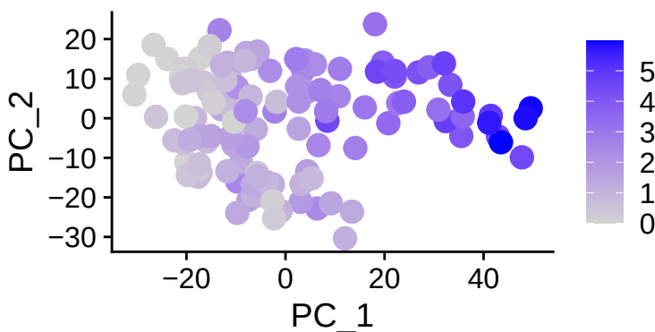
CERS3
