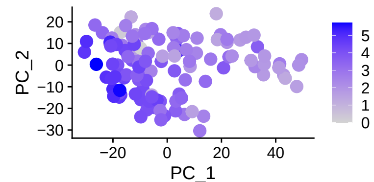
UNC5A
