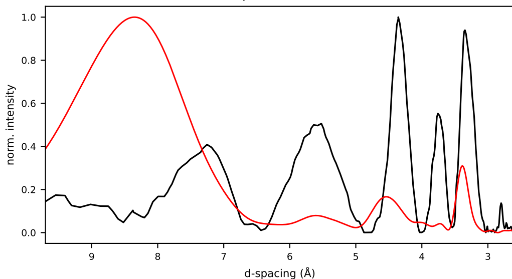
18/cand4/initial.pdb r=-0.167 R_{wp}=1.389 E=\text{nan} kcal/mol
