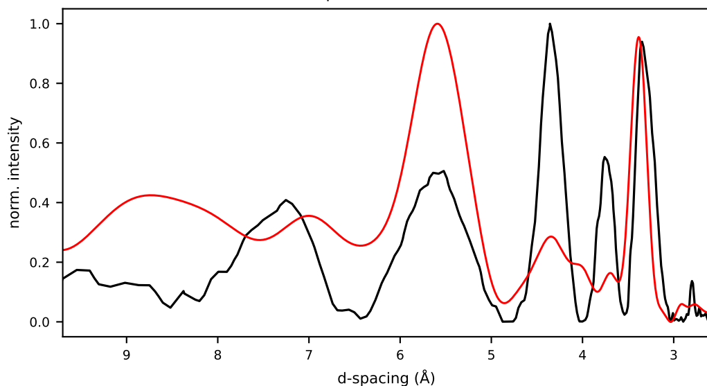
28/cand25/initial.pdb r=0.410 Rwp=0.857 E=-58.4 kcal/mol
