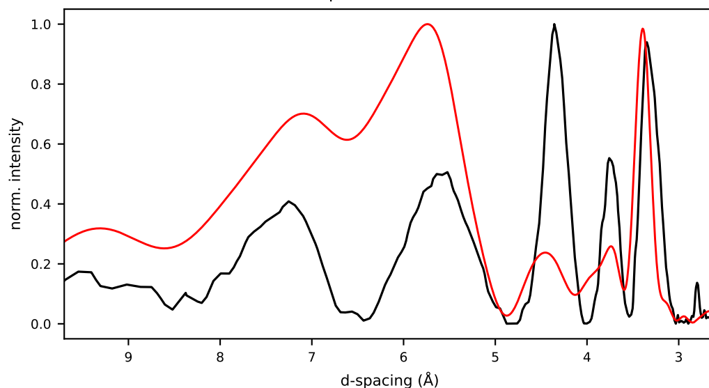
28/cand20/initial.pdb r=0.337 Rwp=1.003 E=-80.1 kcal/mol
