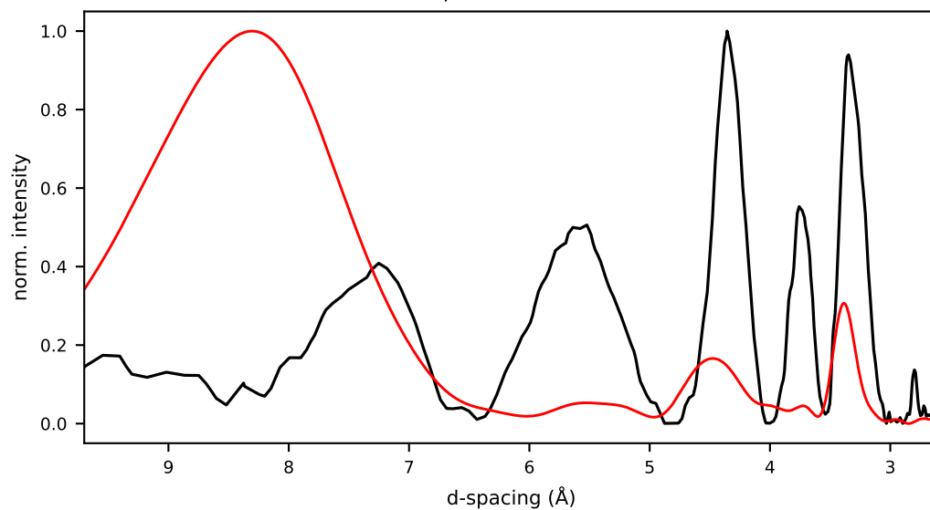
18/cand7/initial.pdb r=-0.159 R_{wp}=1.383 E=\text{nan} kcal/mol
