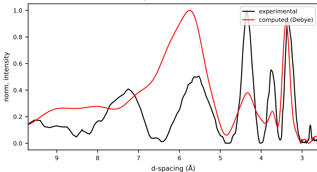
28/cand7/initial.pdb r=0.477 Rwp=0.828 E=-118.5 kcal/mol
