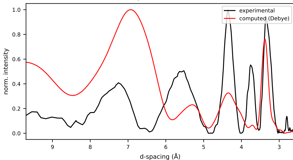
18/cand2/initial.pdb r=-0.174 R_{wp}=1.395 E=\text{nan} kcal/mol
