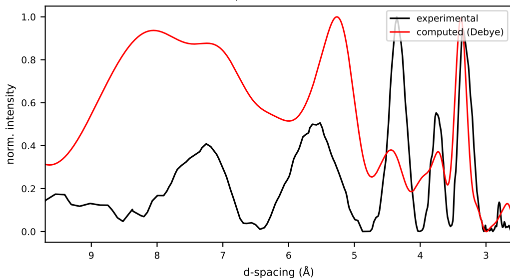
32/cand0/initial.pdb r=0.425 Rwp=0.901 E=-100.6 kcal/mol
