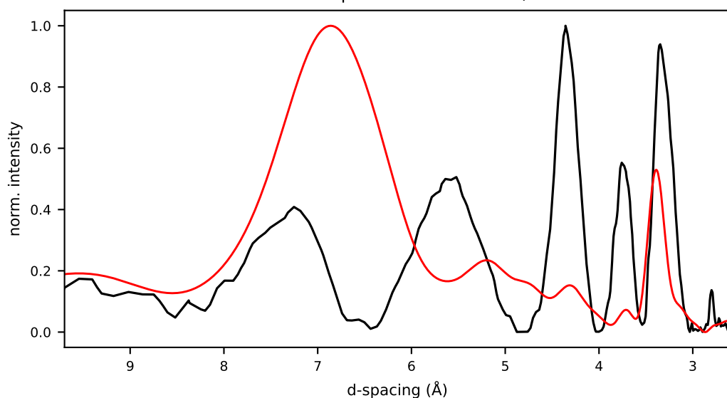
25/cand0/initial.pdb r=0.018 Rwp=1.101 E=-149.5 kcal/mol
