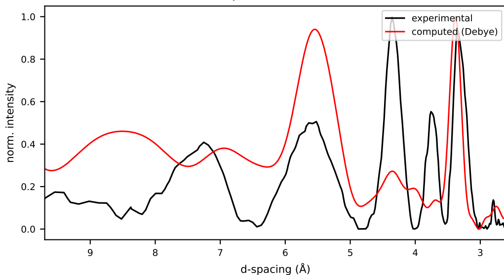
29/cand1/initial.pdb r=0.332 Rwp=0.918 E=-132.8 kcal/mol
