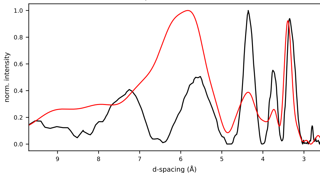
28/cand8/initial.pdb r=0.355 Rwp=1.020 E=-118.3 kcal/mol
