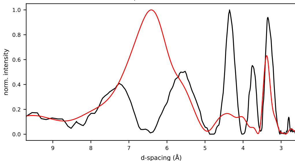
27/cand7/initial.pdb r=0.151 Rwp=1.147 E=-112.4 kcal/mol
