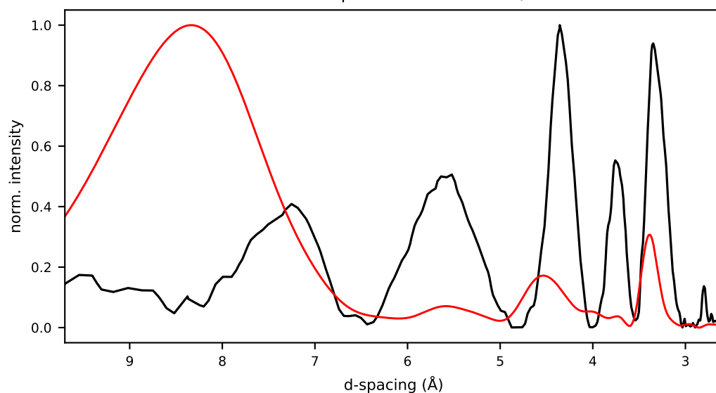
18/cand11/initial.pdb r=-0.166 R_{wp}=1.384 E=\text{nan} kcal/mol
