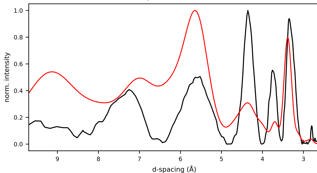
28/cand0/initial.pdb r=0.186 Rwp=1.053 E=-140.9 kcal/mol
