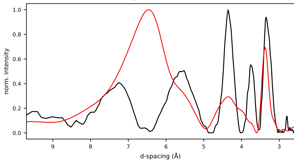
27/cand2/initial.pdb r=0.120 Rwp=1.067 E=-139.4 kcal/mol
