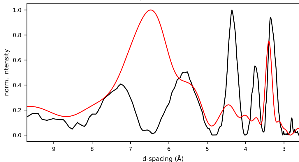
27/cand0/initial.pdb r=0.097 Rwp=1.079 E=-146.2 kcal/mol
