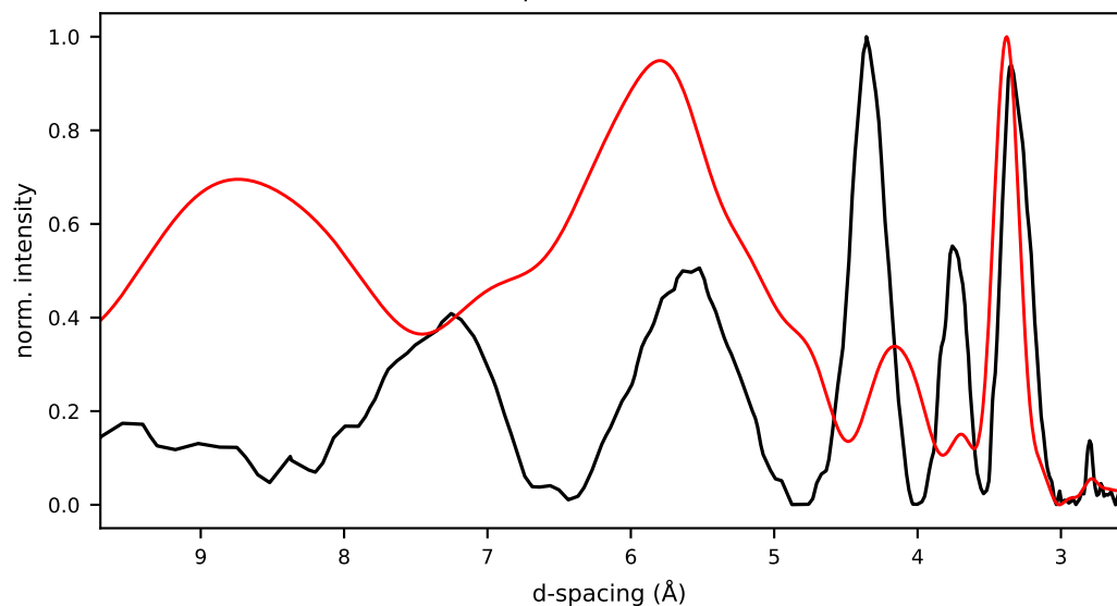
26/cand0/initial.pdb r=0.077 Rwp=1.106 E=nan kcal/mol
