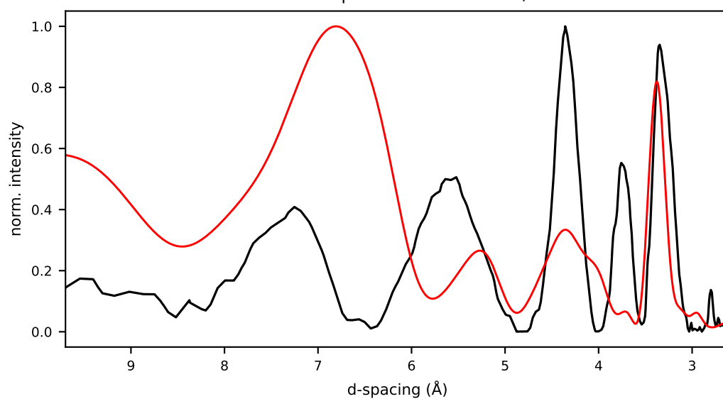
19/cand0/initial.pdb r=0.051 R_{wp}=1.183 E=\text{nan} kcal/mol
