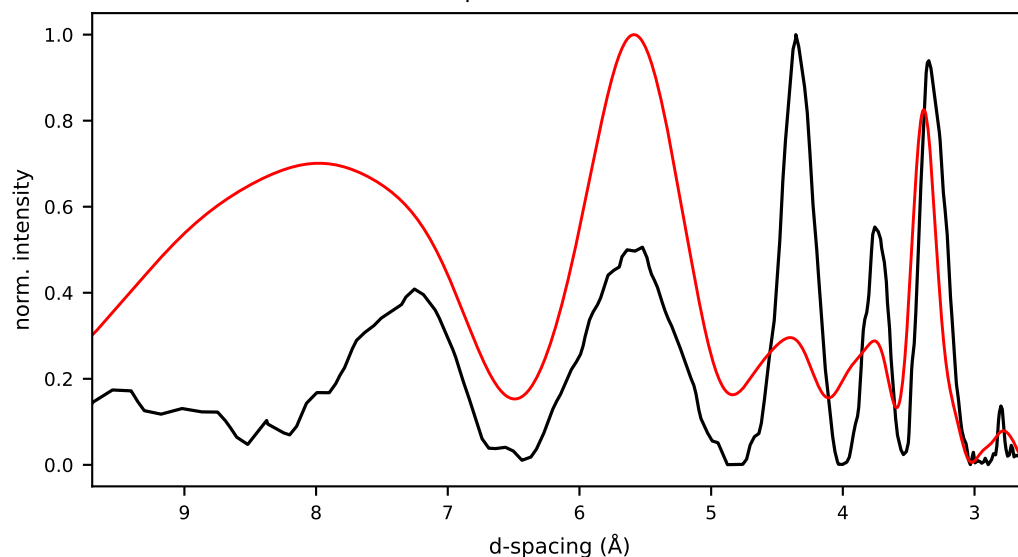
31/cand11/initial.pdb r=0.279 Rwp=1.290 E=-91.1 kcal/mol
