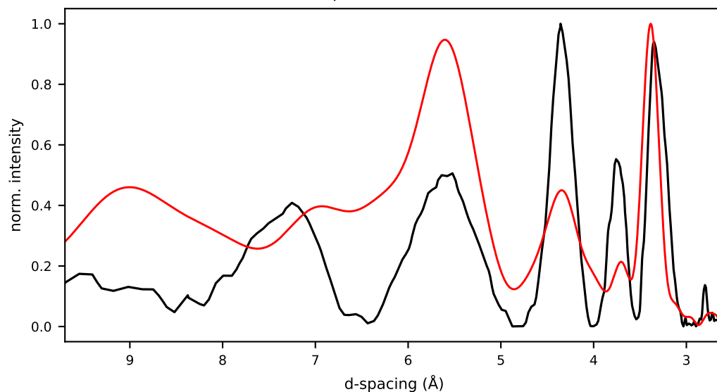
27/cand22/initial.pdb r=0.410 Rwp=1.014 E=-61.8 kcal/mol
