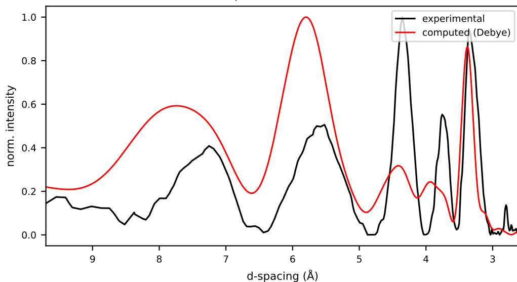
30/cand2/initial.pdb r=0.424 Rwp=0.832 E=-131.6 kcal/mol
