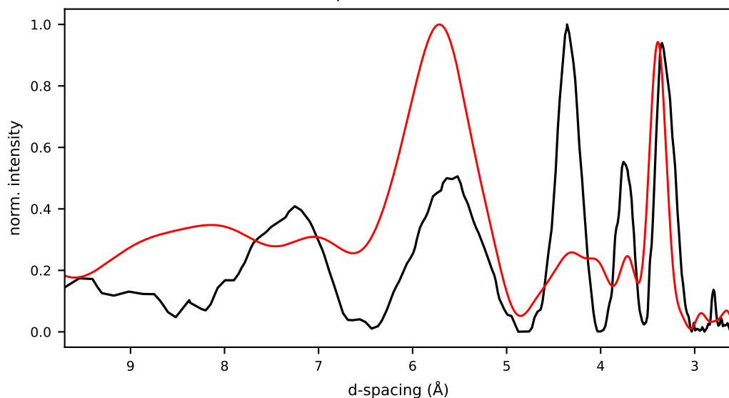
29/cand11/initial.pdb r=0.330 Rwp=1.054 E=-69.9 kcal/mol
