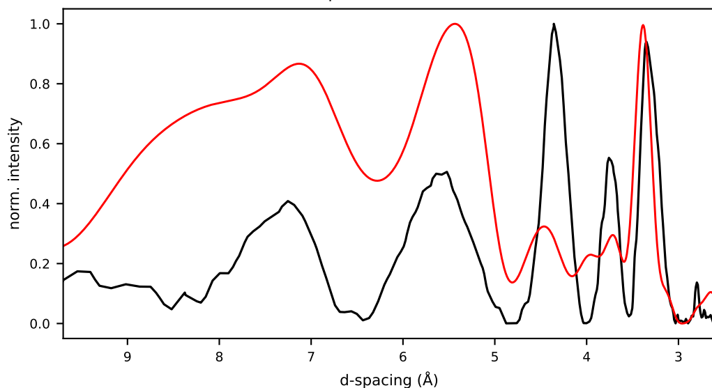
31/cand0/initial.pdb r=0.427 Rwp=0.882 E=-130.1 kcal/mol
