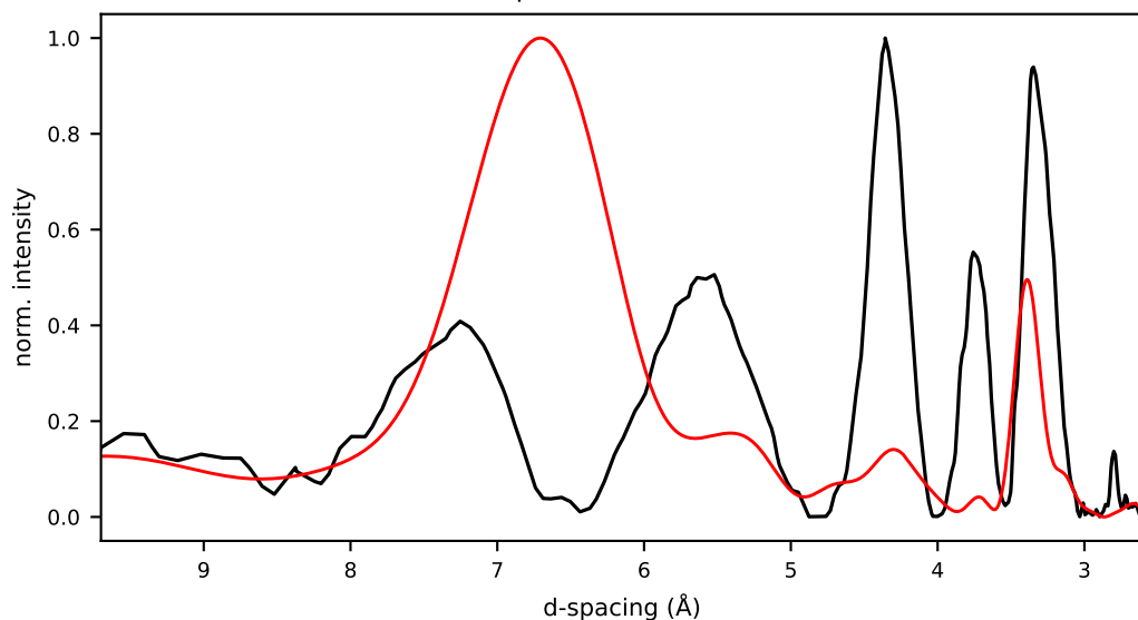
25/cand8/initial.pdb r=0.002 Rwp=1.109 E=-126.1 kcal/mol
