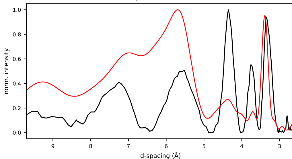
27/cand16/initial.pdb r=0.255 Rwp=1.132 E=-92.6 kcal/mol
