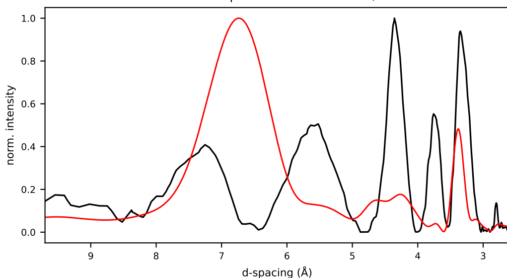
25/cand2/initial.pdb r=0.012 Rwp=1.114 E=-143.3 kcal/mol
