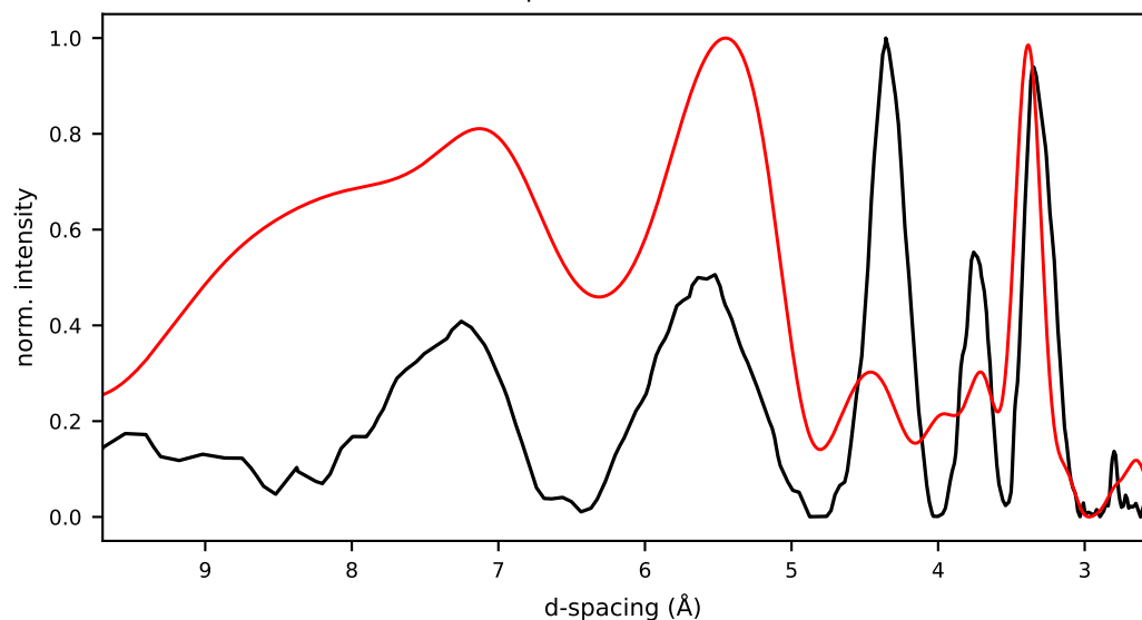
31/cand1/initial.pdb r=0.464 Rwp=0.833 E=-125.8 kcal/mol
