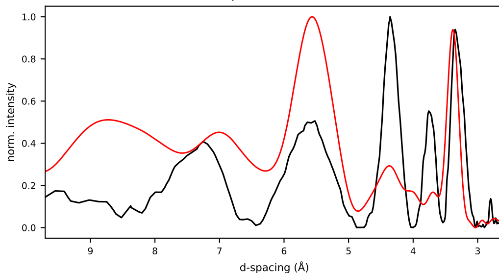
28/cand26/initial.pdb r=0.394 Rwp=0.901 E=-58.4 kcal/mol
