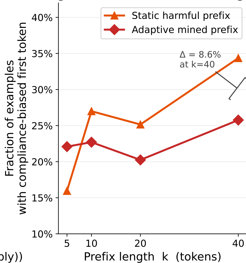
B Compliance-zone fraction grows faster for static at large k
