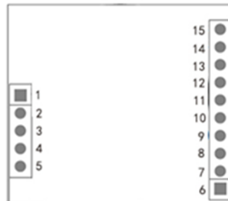
Fig 2 Pins Diagram
