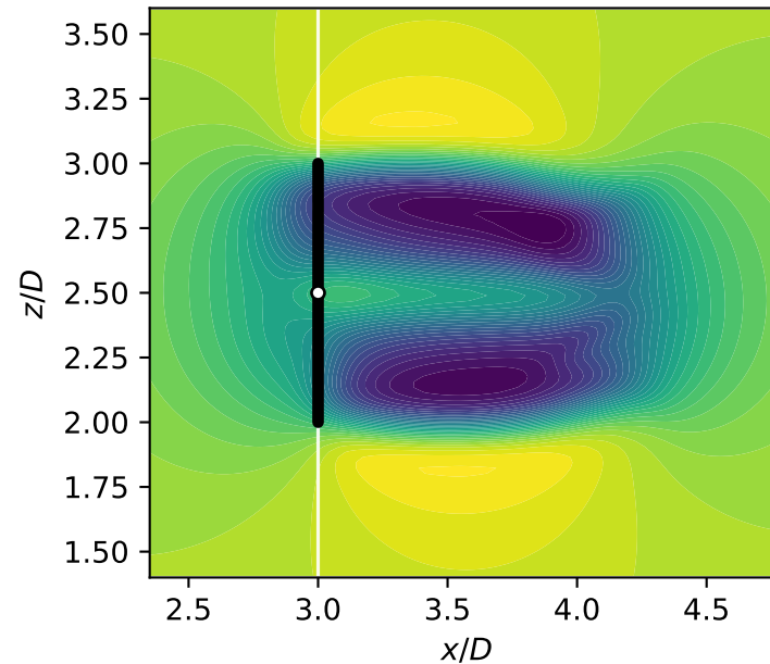
(b) GPU backend: axial velocity u/U_\infty
