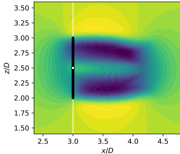
(a) CPU backend: axial velocity u/U_\infty
