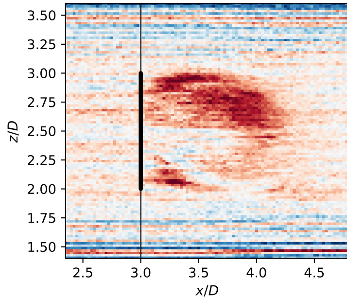
(c) GPU minus CPU (roundoff scale)
